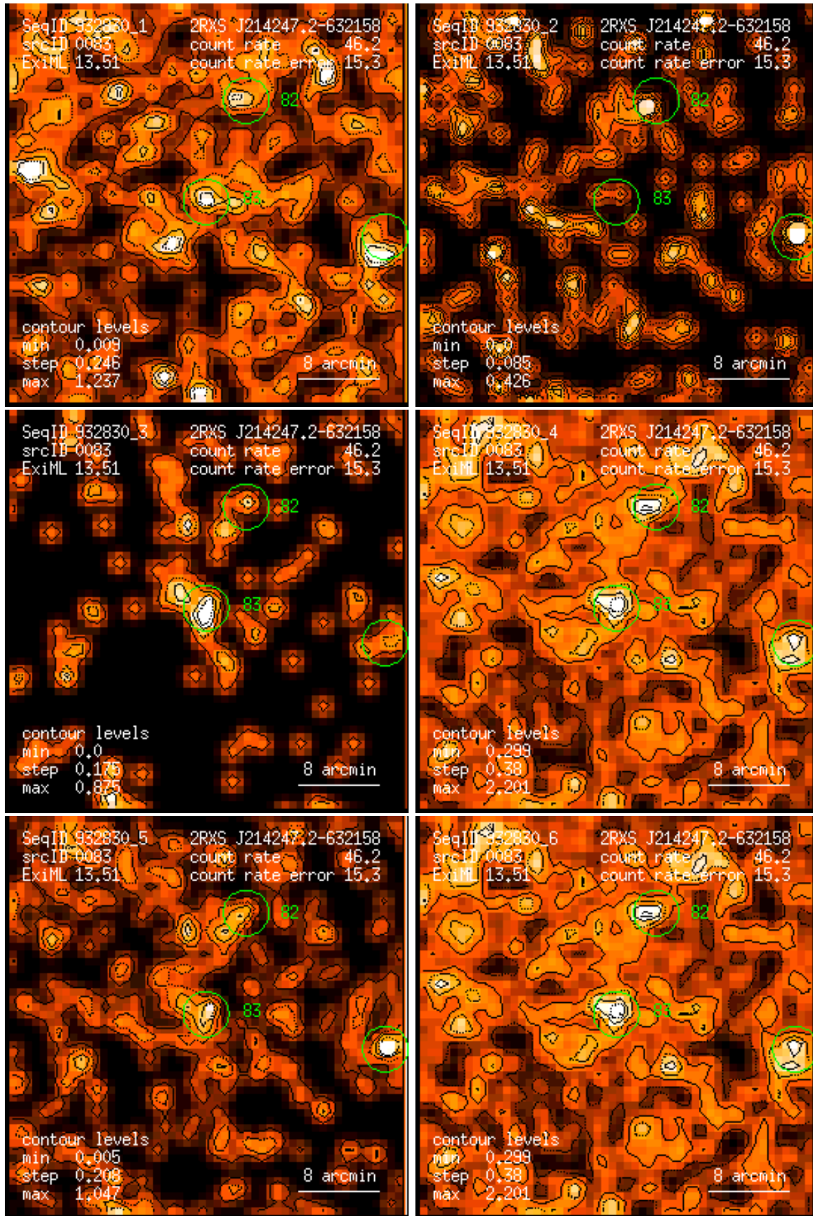
Figure 83: RASS 932830: detection 0083: band rate images, Gaussian filter: (1) PSPC channels 11 – 41, (2) 52 – 90, (3) 91 – 201, (4) 11 – 235, (5) 52 – 201, (6) 11 – 201. Broad band rates in counts/ks. Band rate contour levels in counts/ks/arcmin 2 .
