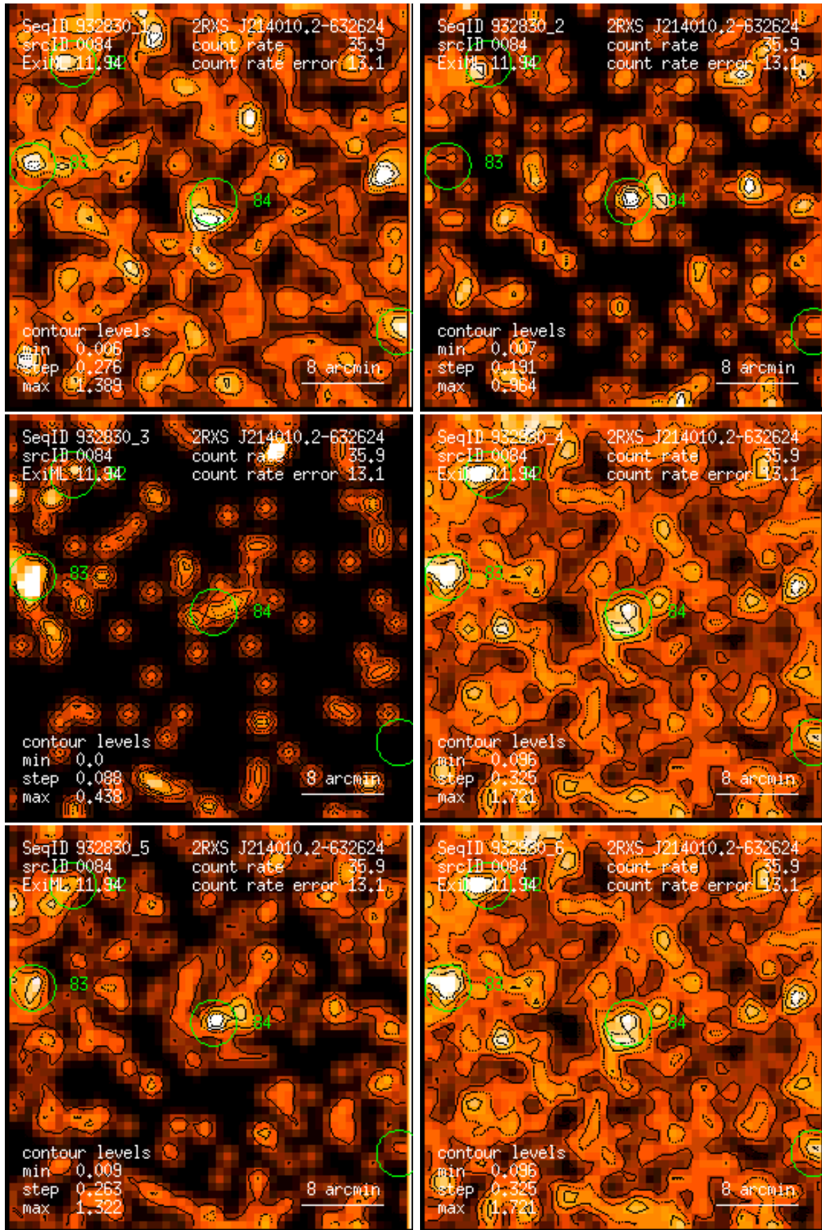
Figure 84: RASS 932830: detection 0084: band rate images, Gaussian filter: (1) PSPC channels 11 – 41, (2) 52 – 90, (3) 91 – 201, (4) 11 – 235, (5) 52 – 201, (6) 11 – 201. Broad band rates in counts/ks. Band rate contour levels in counts/ks/arcmin 2 .
