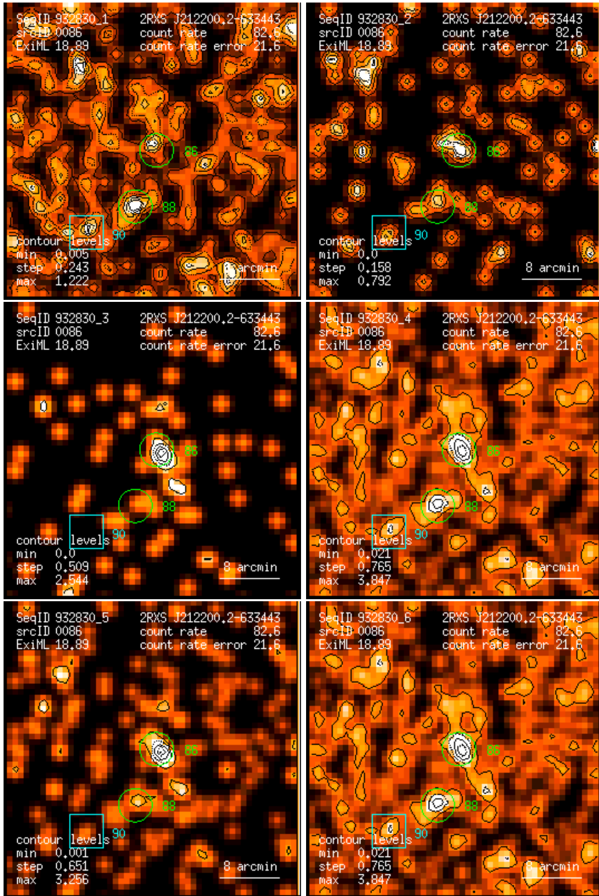
Figure 86: RASS 932830: detection 0086: band rate images, Gaussian filter: (1) PSPC channels 11 – 41, (2) 52 – 90, (3) 91 – 201, (4) 11 – 235, (5) 52 – 201, (6) 11 – 201. Broad band rates in counts/ks. Band rate contour levels in counts/ks/arcmin 2 .
