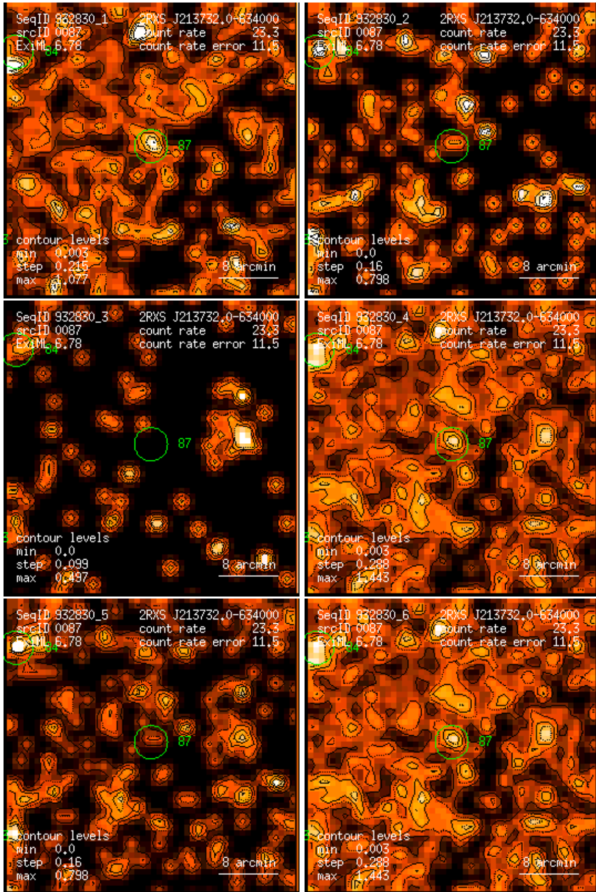
Figure 87: RASS 932830: detection 0087: band rate images, Gaussian filter: (1) PSPC channels 11 – 41, (2) 52 – 90, (3) 91 – 201, (4) 11 – 235, (5) 52 – 201, (6) 11 – 201. Broad band rates in counts/ks. Band rate contour levels in counts/ks/arcmin 2 .
