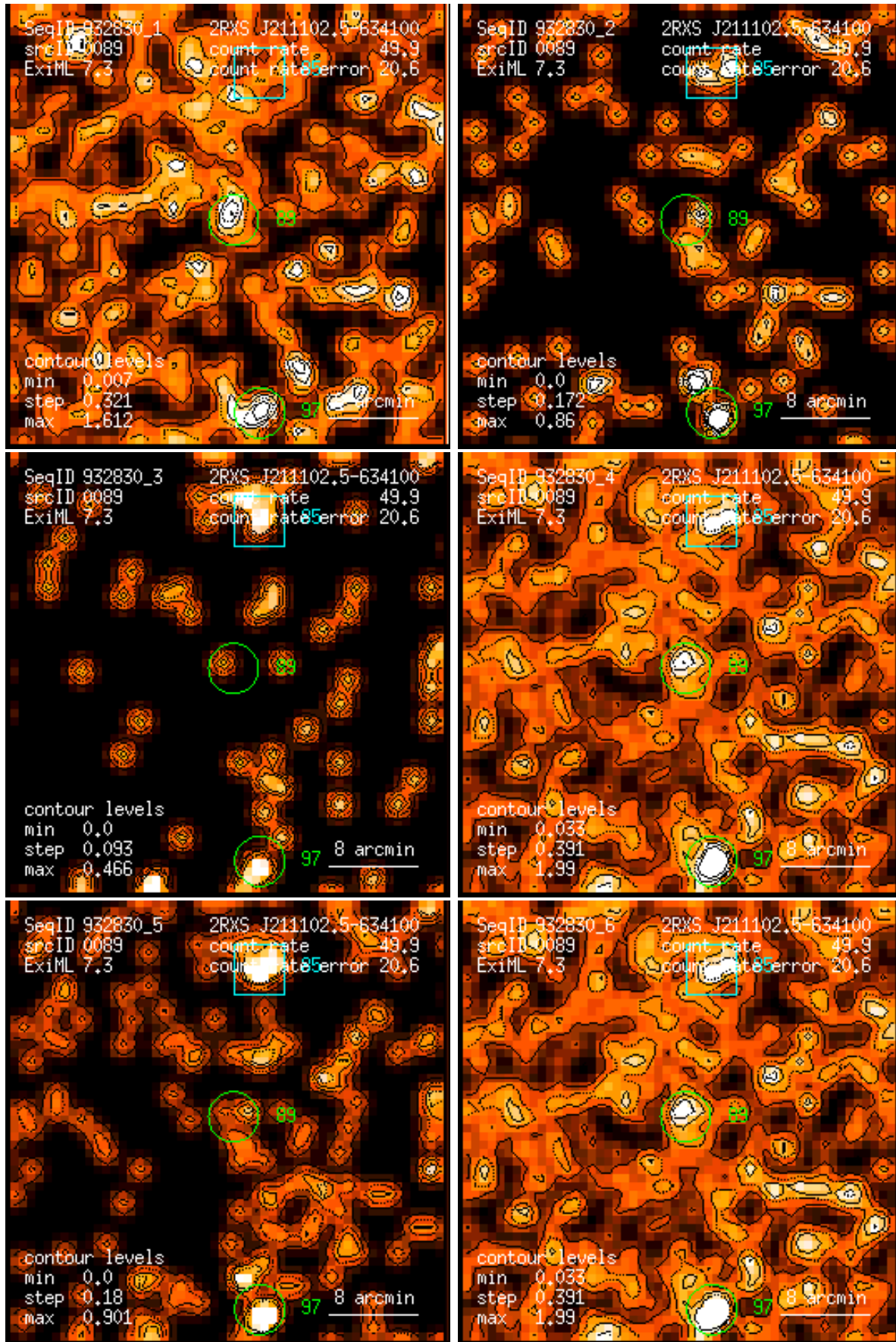
Figure 89: RASS 932830: detection 0089: band rate images, Gaussian filter: (1) PSPC channels 11 – 41, (2) 52 – 90, (3) 91 – 201, (4) 11 – 235, (5) 52 – 201, (6) 11 – 201. Broad band rates in counts/ks. Band rate contour levels in counts/ks/arcmin 2 .
