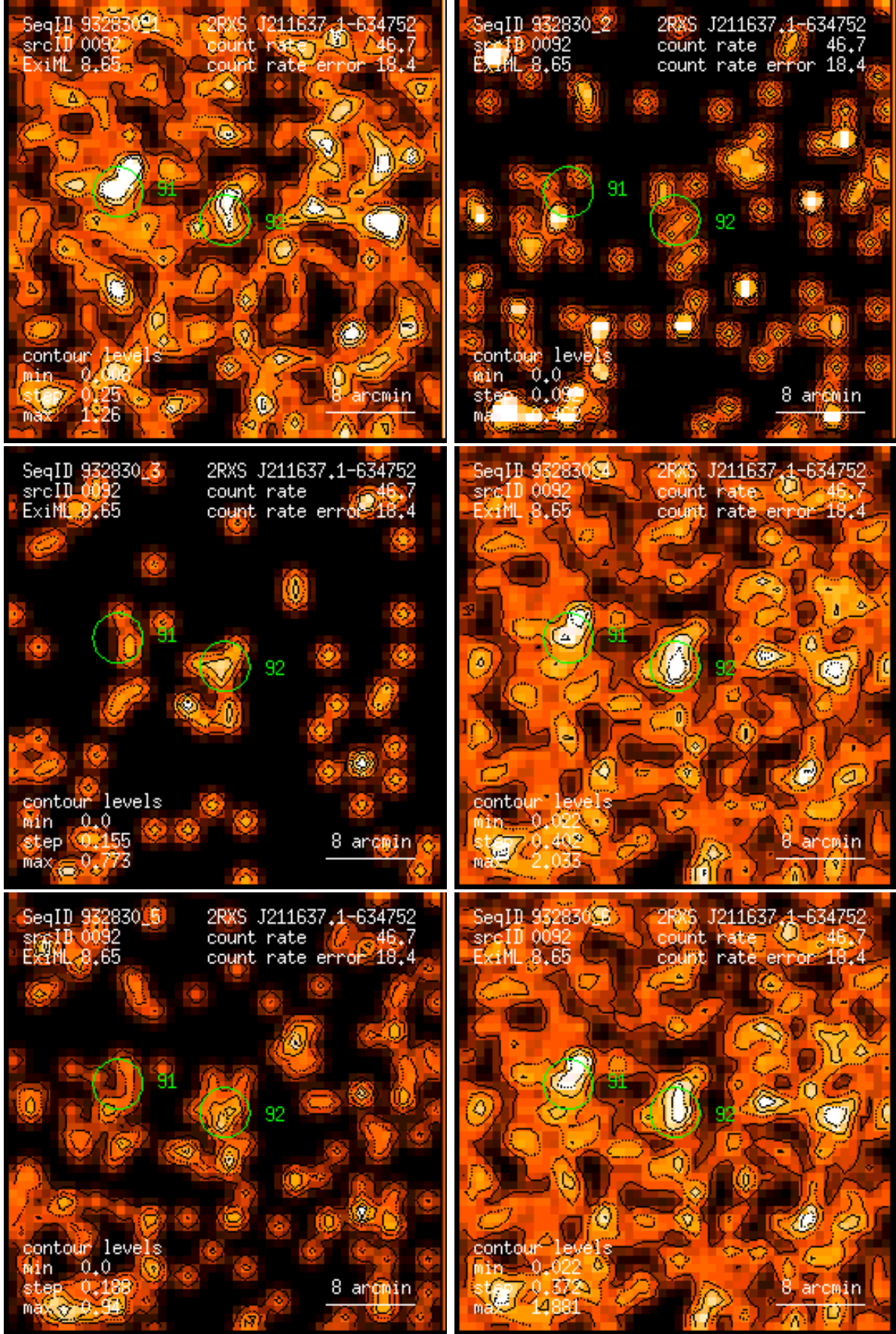
Figure 92: RASS 932830: detection 0092: band rate images, Gaussian filter: (1) PSPC channels 11 – 41, (2) 52 – 90, (3) 91 – 201, (4) 11 – 235, (5) 52 – 201, (6) 11 – 201. Broad band rates in counts/ks. Band rate contour levels in counts/ks/arcmin 2 .
