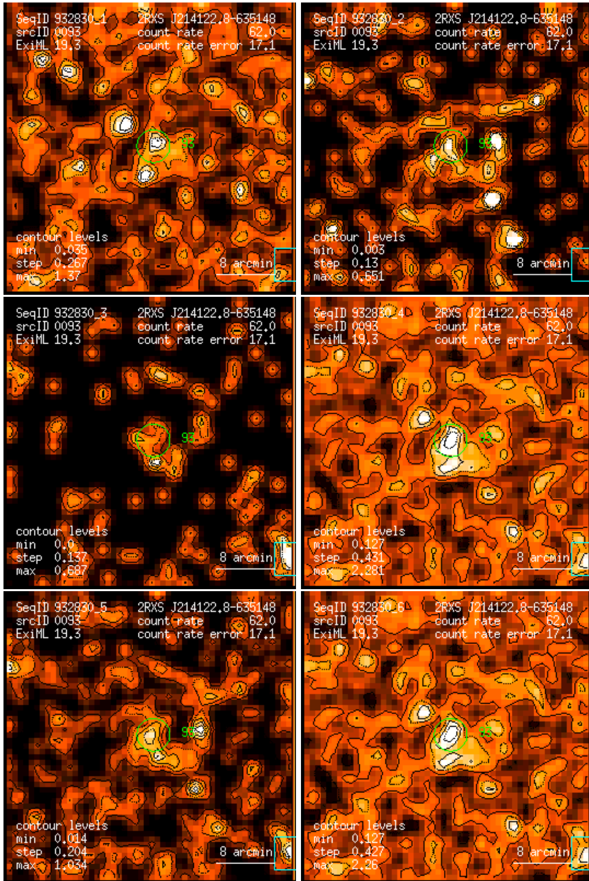
Figure 93: RASS 932830: detection 0093: band rate images, Gaussian filter: (1) PSPC channels 11 – 41, (2) 52 – 90, (3) 91 – 201, (4) 11 – 235, (5) 52 – 201, (6) 11 – 201. Broad band rates in counts/ks. Band rate contour levels in counts/ks/arcmin 2 .
