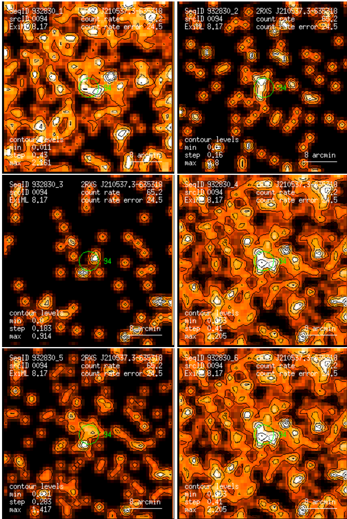
Figure 94: RASS 932830: detection 0094: band rate images, Gaussian filter: (1) PSPC channels 11 – 41, (2) 52 – 90, (3) 91 – 201, (4) 11 – 235, (5) 52 – 201, (6) 11 – 201. Broad band rates in counts/ks. Band rate contour levels in counts/ks/arcmin 2 .
