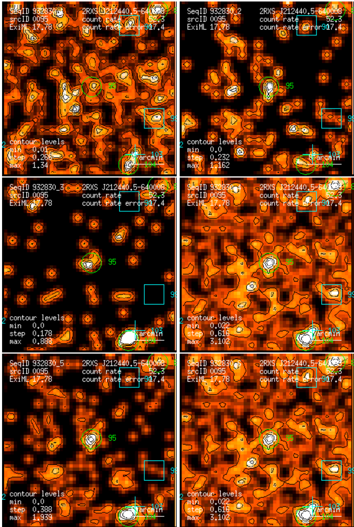
Figure 95: RASS 932830: detection 0095: band rate images, Gaussian filter: (1) PSPC channels 11 – 41, (2) 52 – 90, (3) 91 – 201, (4) 11 – 235, (5) 52 – 201, (6) 11 – 201. Broad band rates in counts/ks. Band rate contour levels in counts/ks/arcmin 2 .
