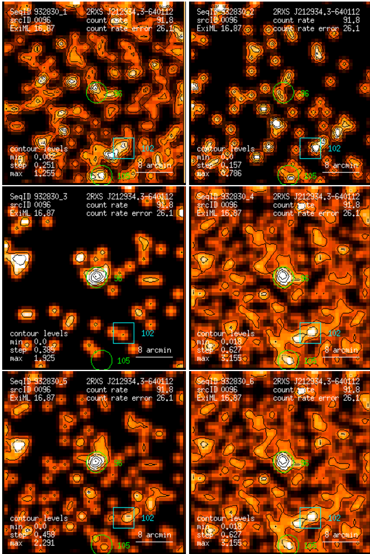
Figure 96: RASS 932830: detection 0096: band rate images, Gaussian filter: (1) PSPC channels 11 – 41, (2) 52 – 90, (3) 91 – 201, (4) 11 – 235, (5) 52 – 201, (6) 11 – 201. Broad band rates in counts/ks. Band rate contour levels in counts/ks/arcmin 2 .
