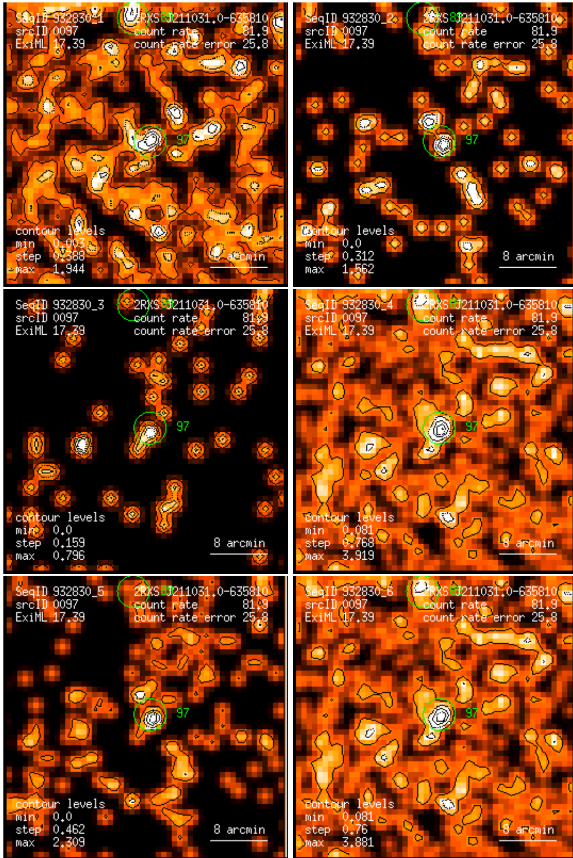
Figure 97: RASS 932830: detection 0097: band rate images, Gaussian filter: (1) PSPC channels 11 – 41, (2) 52 – 90, (3) 91 – 201, (4) 11 – 235, (5) 52 – 201, (6) 11 – 201. Broad band rates in counts/ks. Band rate contour levels in counts/ks/arcmin 2 .
