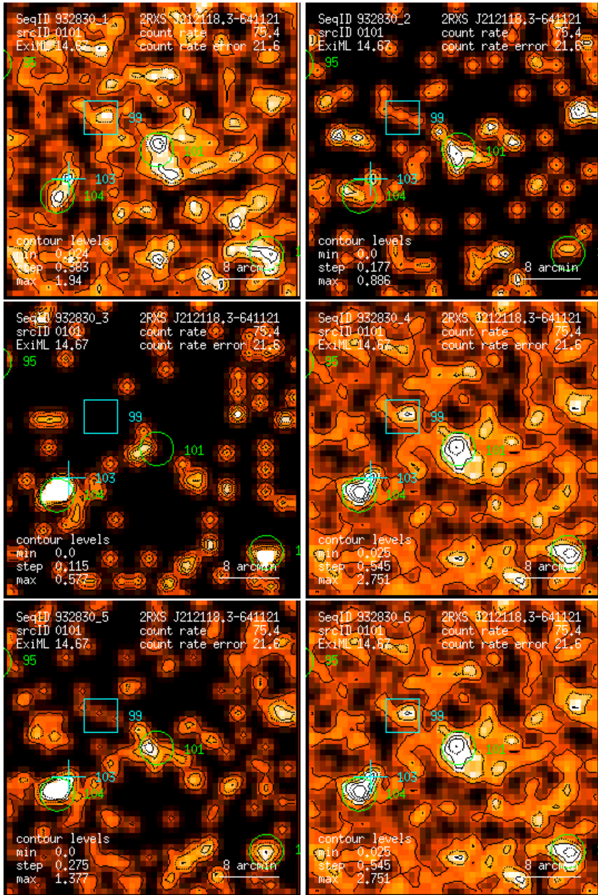
Figure 101: RASS 932830: detection 0101: band rate images, Gaussian filter: (1) PSPC channels 11 – 41, (2) 52 – 90, (3) 91 – 201, (4) 11 – 235, (5) 52 – 201, (6) 11 – 201. Broad band rates in counts/ks. Band rate contour levels in counts/ks/arcmin 2 .
