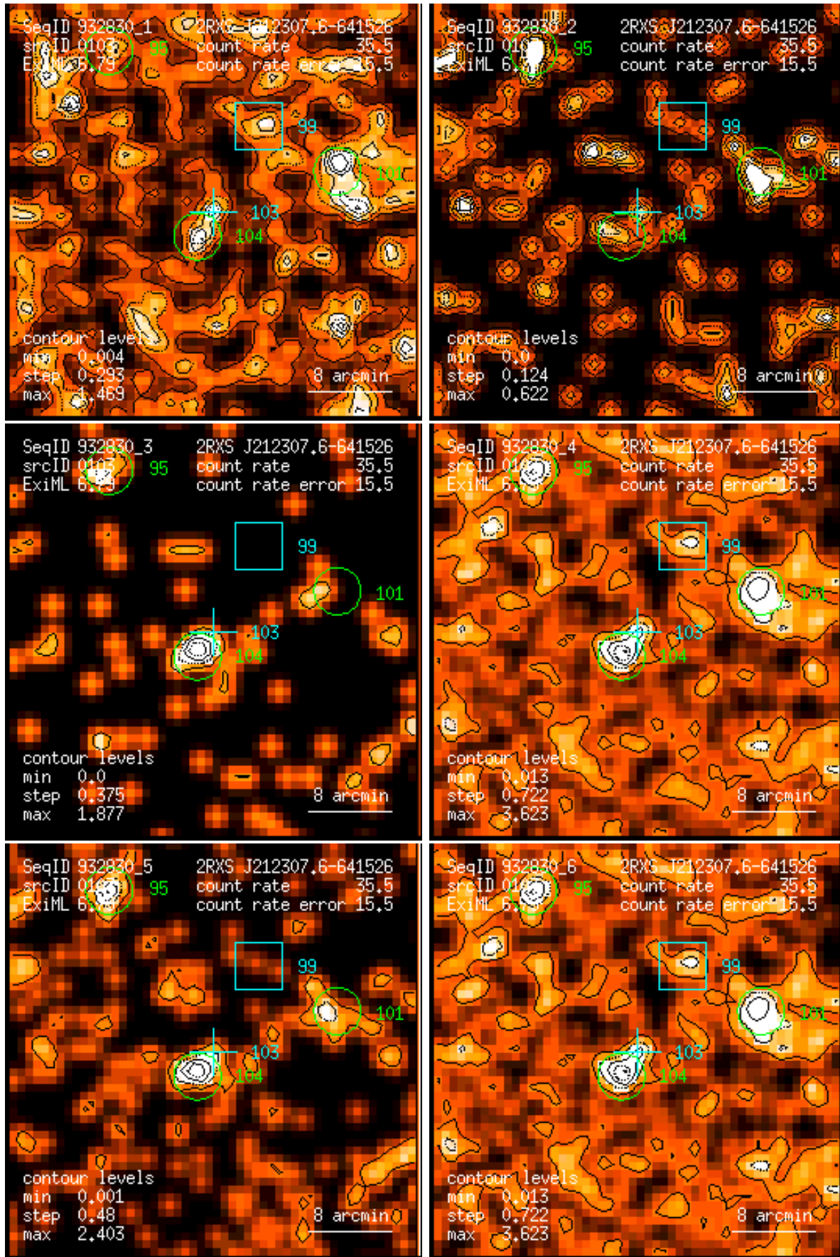
Figure 103: RASS 932830: detection 0103: band rate images, Gaussian filter: (1) PSPC channels 11 – 41, (2) 52 – 90, (3) 91 – 201, (4) 11 – 235, (5) 52 – 201, (6) 11 – 201. Broad band rates in counts/ks. Band rate contour levels in counts/ks/arcmin 2 .
