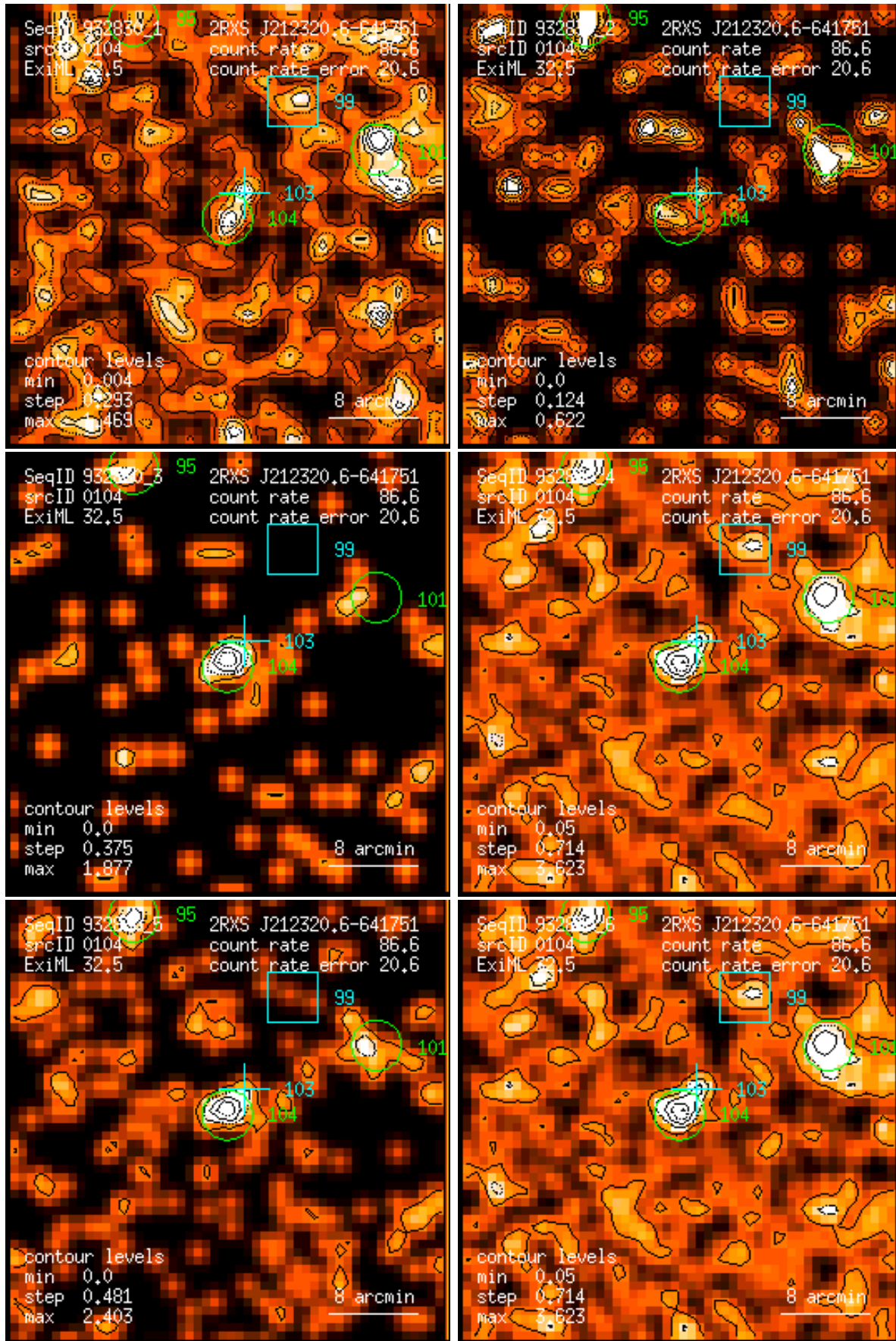
Figure 104: RASS 932830: detection 0104: band rate images, Gaussian filter: (1) PSPC channels 11 – 41, (2) 52 – 90, (3) 91 – 201, (4) 11 – 235, (5) 52 – 201, (6) 11 – 201. Broad band rates in counts/ks. Band rate contour levels in counts/ks/arcmin 2 .
