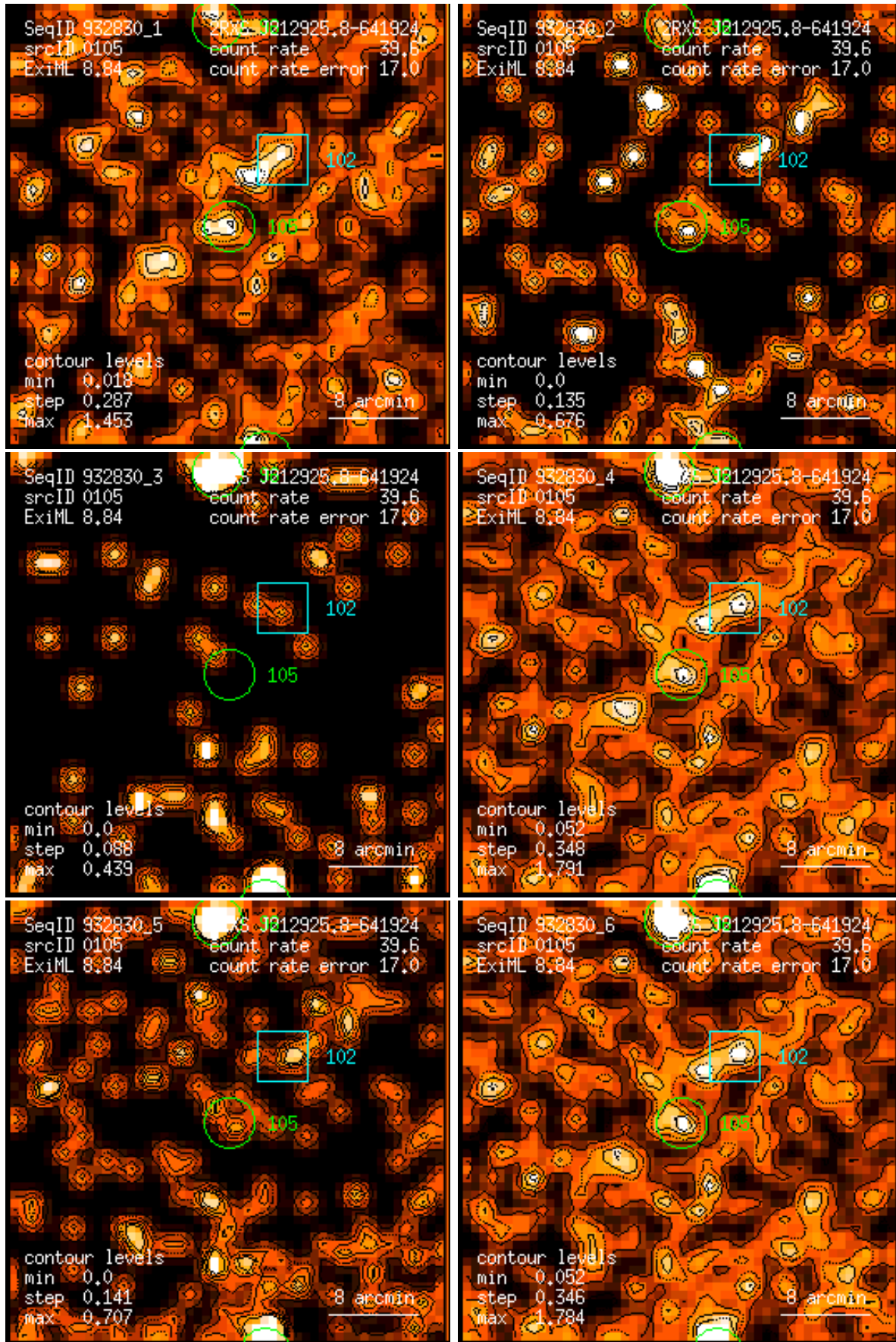
Figure 105: RASS 932830: detection 0105: band rate images, Gaussian filter: (1) PSPC channels 11 – 41, (2) 52 – 90, (3) 91 – 201, (4) 11 – 235, (5) 52 – 201, (6) 11 – 201. Broad band rates in counts/ks. Band rate contour levels in counts/ks/arcmin 2 .
