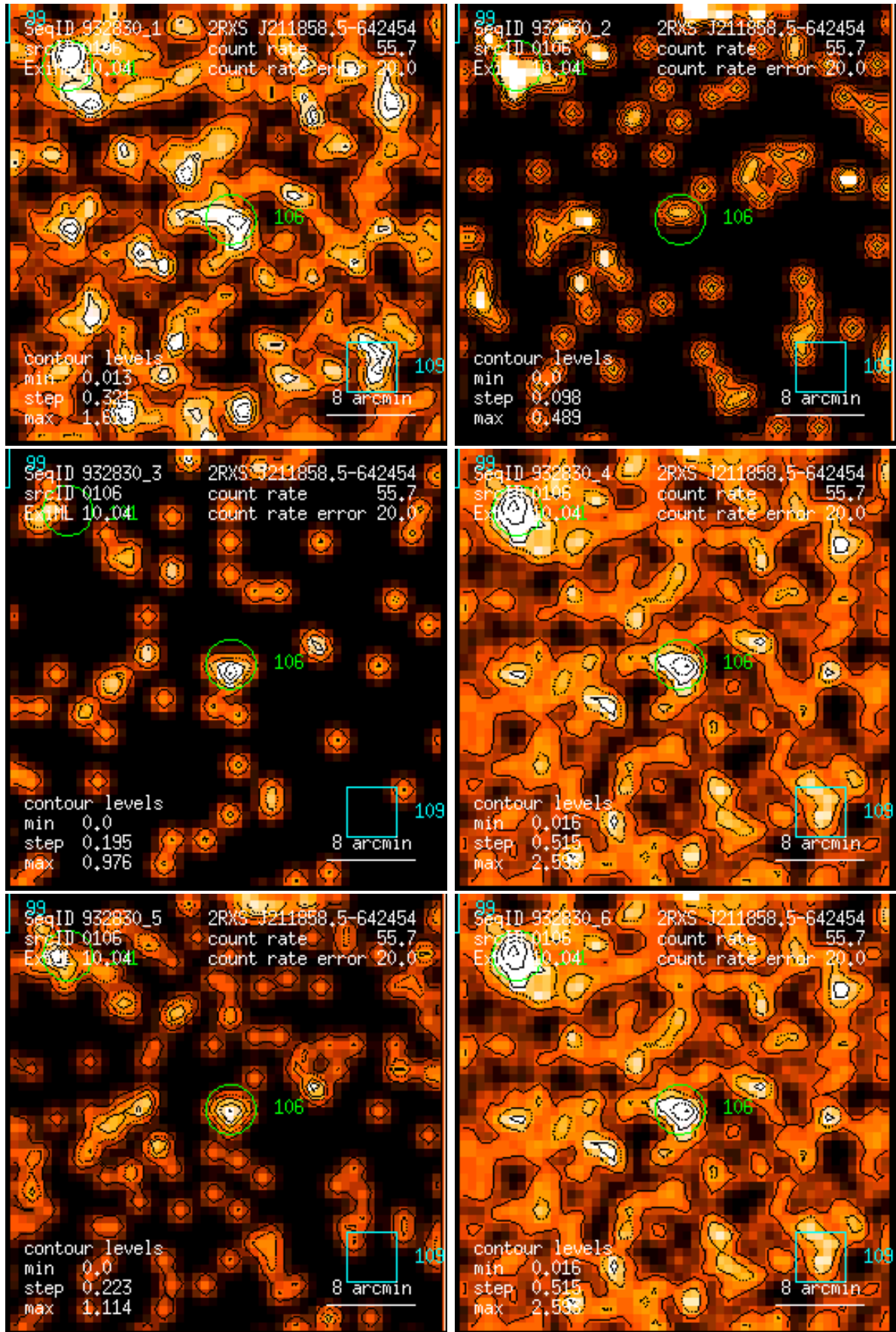
Figure 106: RASS 932830: detection 0106: band rate images, Gaussian filter: (1) PSPC channels 11 – 41, (2) 52 – 90, (3) 91 – 201, (4) 11 – 235, (5) 52 – 201, (6) 11 – 201. Broad band rates in counts/ks. Band rate contour levels in counts/ks/arcmin 2 .
