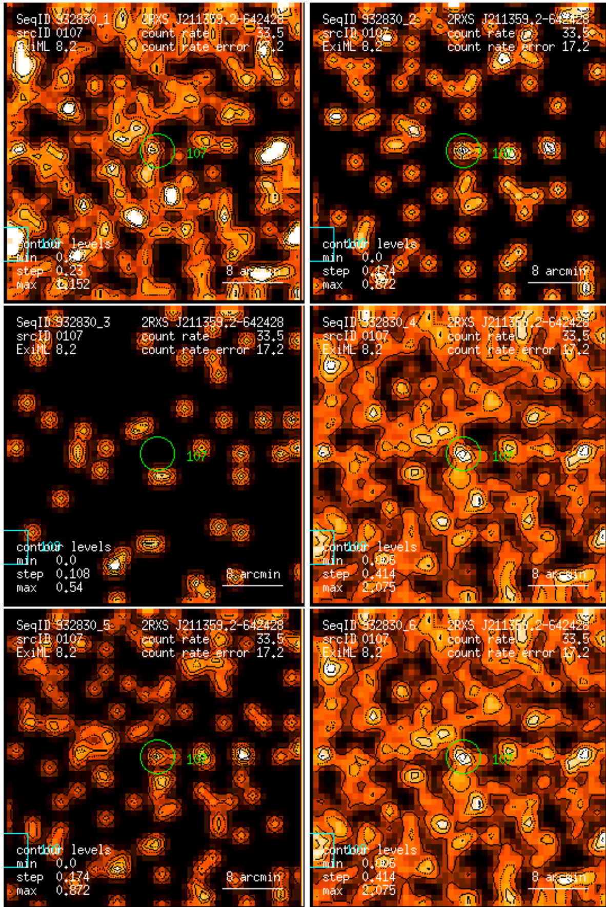
Figure 107: RASS 932830: detection 0107: band rate images, Gaussian filter: (1) PSPC channels 11 – 41, (2) 52 – 90, (3) 91 – 201, (4) 11 – 235, (5) 52 – 201, (6) 11 – 201. Broad band rates in counts/ks. Band rate contour levels in counts/ks/arcmin 2 .
