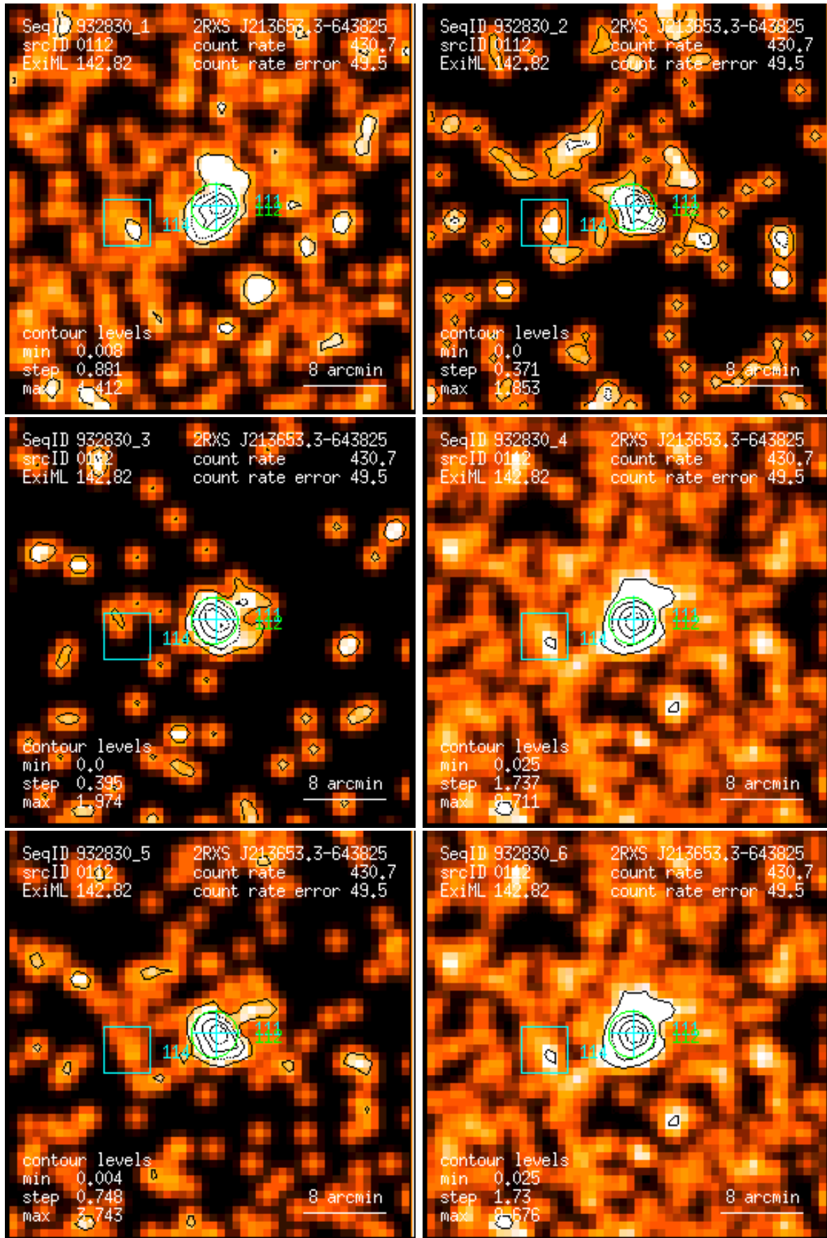
Figure 112: RASS 932830: detection 0112: band rate images, Gaussian filter: (1) PSPC channels 11 – 41, (2) 52 – 90, (3) 91 – 201, (4) 11 – 235, (5) 52 – 201, (6) 11 – 201. Broad band rates in counts/ks. Band rate contour levels in counts/ks/arcmin 2 .
