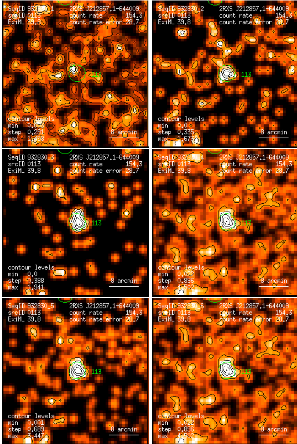
Figure 113: RASS 932830: detection 0113: band rate images, Gaussian filter: (1) PSPC channels 11 – 41, (2) 52 – 90, (3) 91 – 201, (4) 11 – 235, (5) 52 – 201, (6) 11 – 201. Broad band rates in counts/ks. Band rate contour levels in counts/ks/arcmin 2 .
