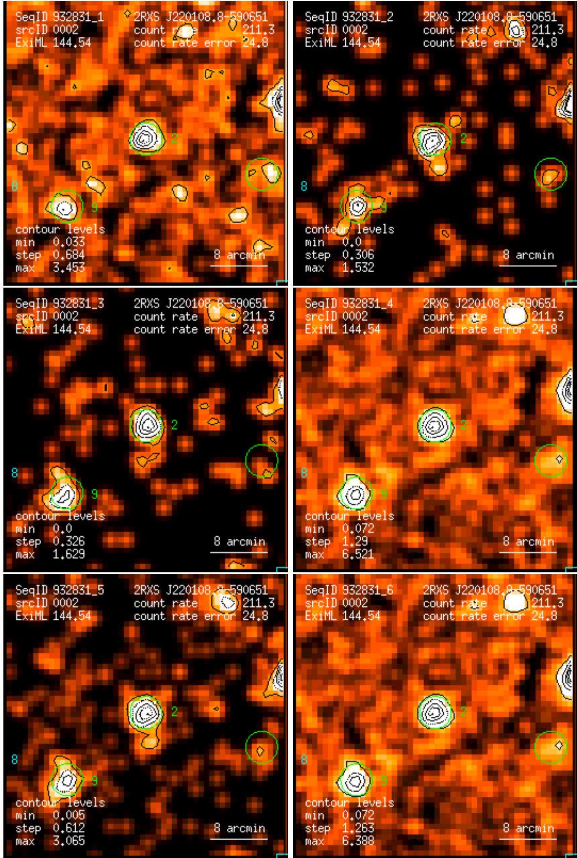
Figure 2: RASS 932831: detection 0002: band rate images, Gaussian filter: (1) PSPC channels 11 – 41, (2) 52 – 90, (3) 91 – 201, (4) 11 – 235, (5) 52 – 201, (6) 11 – 201. Broad band rates in counts/ks. Band rate contour levels in counts/ks/arcmin 2 .
