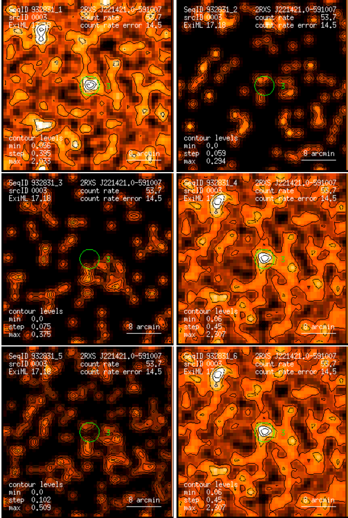
Figure 3: RASS 932831: detection 0003: band rate images, Gaussian filter: (1) PSPC channels 11 – 41, (2) 52 – 90, (3) 91 – 201, (4) 11 – 235, (5) 52 – 201, (6) 11 – 201. Broad band rates in counts/ks. Band rate contour levels in counts/ks/arcmin 2 .
