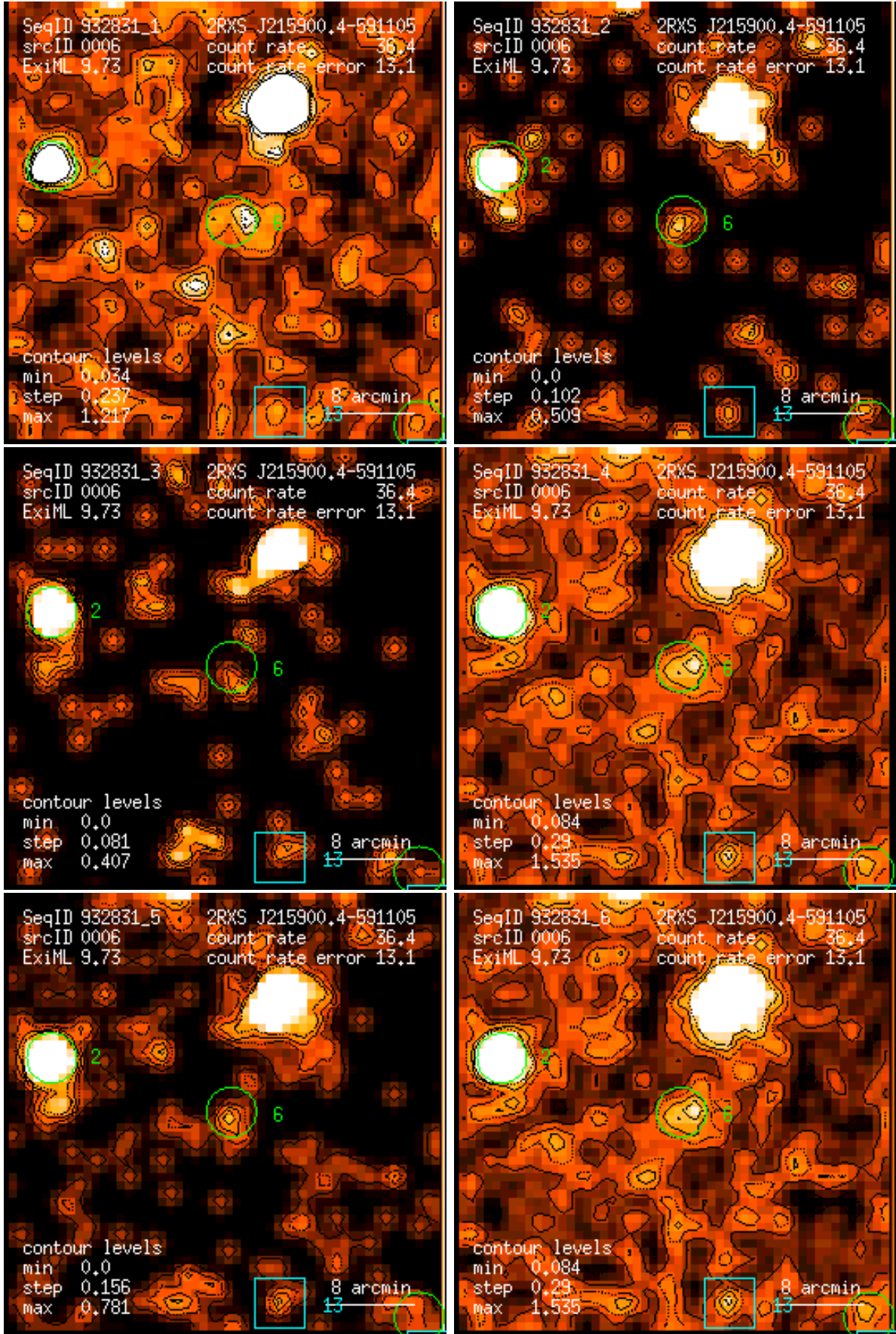
Figure 6: RASS 932831: detection 0006: band rate images, Gaussian filter: (1) PSPC channels 11 – 41, (2) 52 – 90, (3) 91 – 201, (4) 11 – 235, (5) 52 – 201, (6) 11 – 201. Broad band rates in counts/ks. Band rate contour levels in counts/ks/arcmin 2 .
