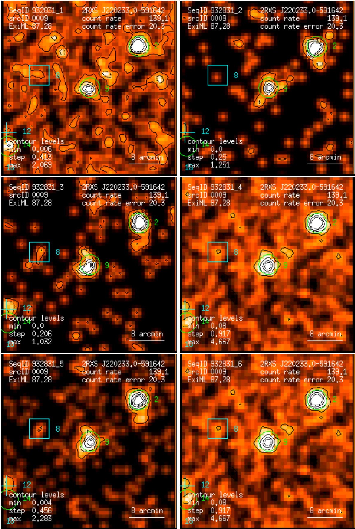
Figure 9: RASS 932831: detection 0009: band rate images, Gaussian filter: (1) PSPC channels 11 – 41, (2) 52 – 90, (3) 91 – 201, (4) 11 – 235, (5) 52 – 201, (6) 11 – 201. Broad band rates in counts/ks. Band rate contour levels in counts/ks/arcmin 2 .
