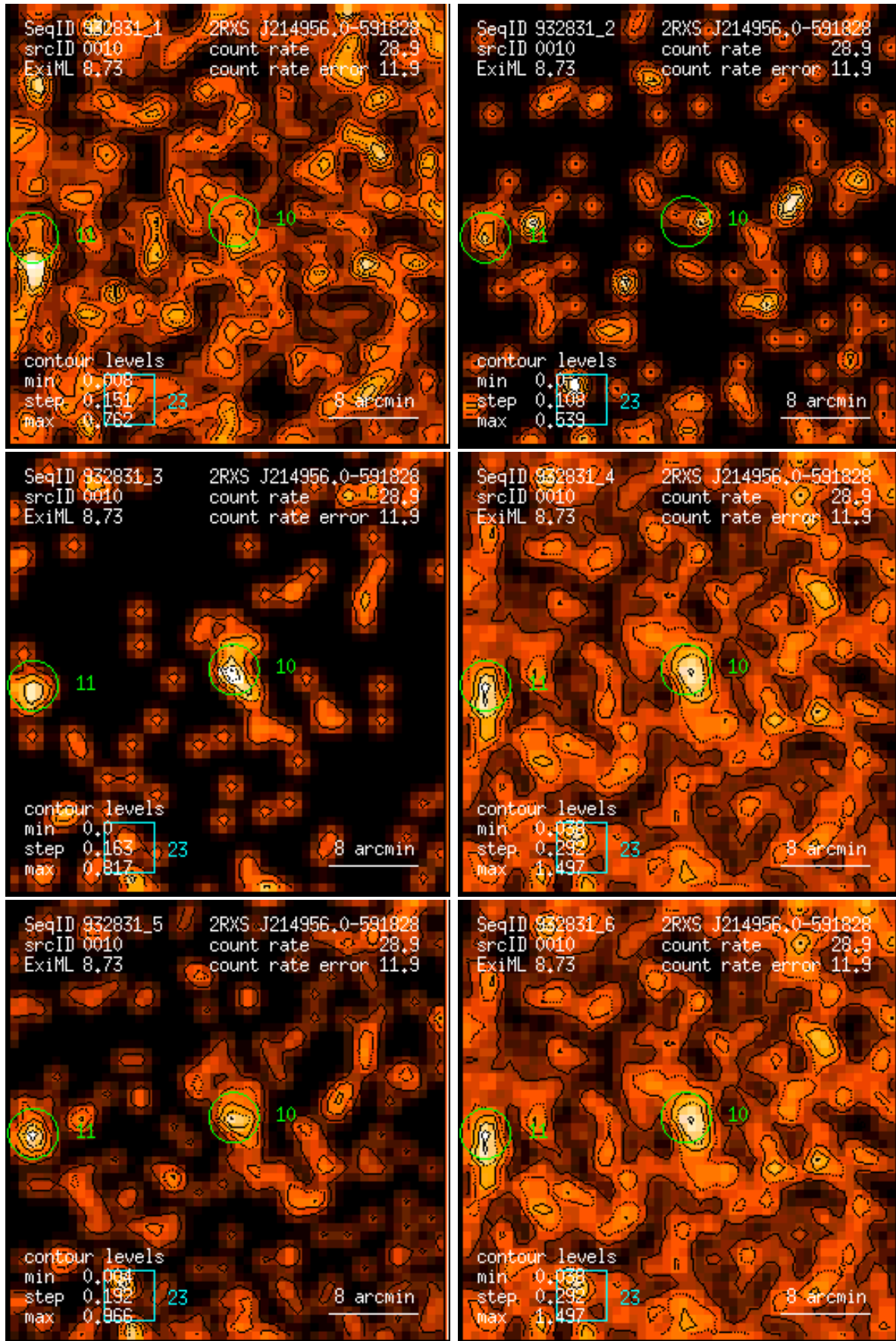
Figure 10: RASS 932831: detection 0010: band rate images, Gaussian filter: (1) PSPC channels 11 – 41, (2) 52 – 90, (3) 91 – 201, (4) 11 – 235, (5) 52 – 201, (6) 11 – 201. Broad band rates in counts/ks. Band rate contour levels in counts/ks/arcmin 2 .
