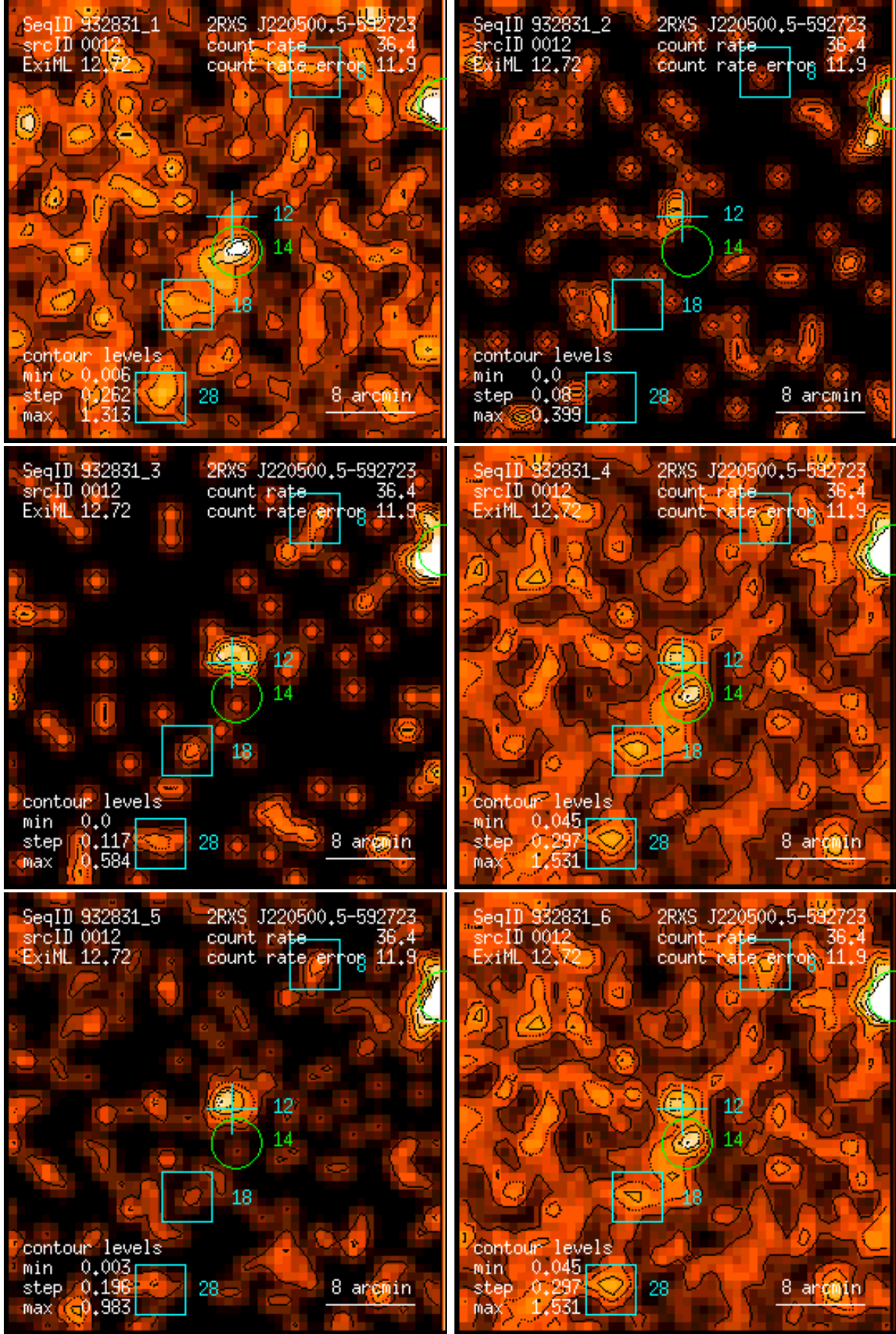
Figure 12: RASS 932831: detection 0012: band rate images, Gaussian filter: (1) PSPC channels 11 – 41, (2) 52 – 90, (3) 91 – 201, (4) 11 – 235, (5) 52 – 201, (6) 11 – 201. Broad band rates in counts/ks. Band rate contour levels in counts/ks/arcmin 2 .
