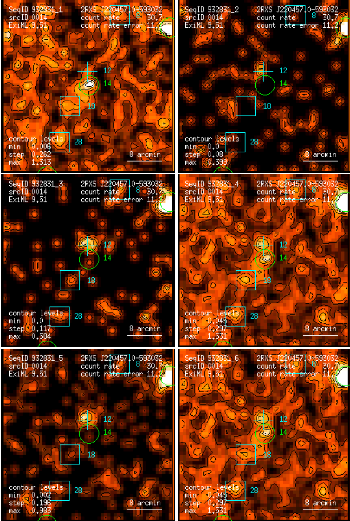
Figure 14: RASS 932831: detection 0014: band rate images, Gaussian filter: (1) PSPC channels 11 – 41, (2) 52 – 90, (3) 91 – 201, (4) 11 – 235, (5) 52 – 201, (6) 11 – 201. Broad band rates in counts/ks. Band rate contour levels in counts/ks/arcmin 2 .
