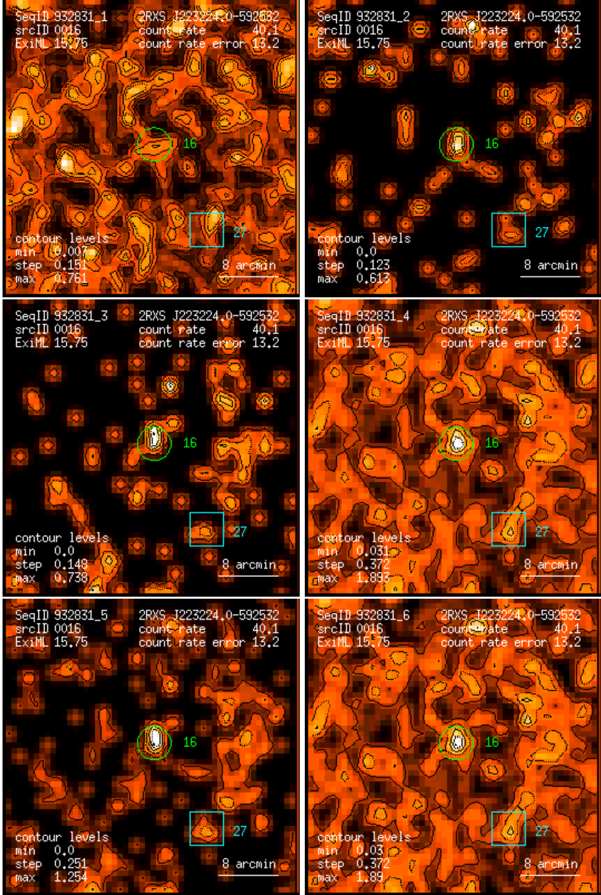
Figure 16: RASS 932831: detection 0016: band rate images, Gaussian filter: (1) PSPC channels 11 – 41, (2) 52 – 90, (3) 91 – 201, (4) 11 – 235, (5) 52 – 201, (6) 11 – 201. Broad band rates in counts/ks. Band rate contour levels in counts/ks/arcmin 2 .
