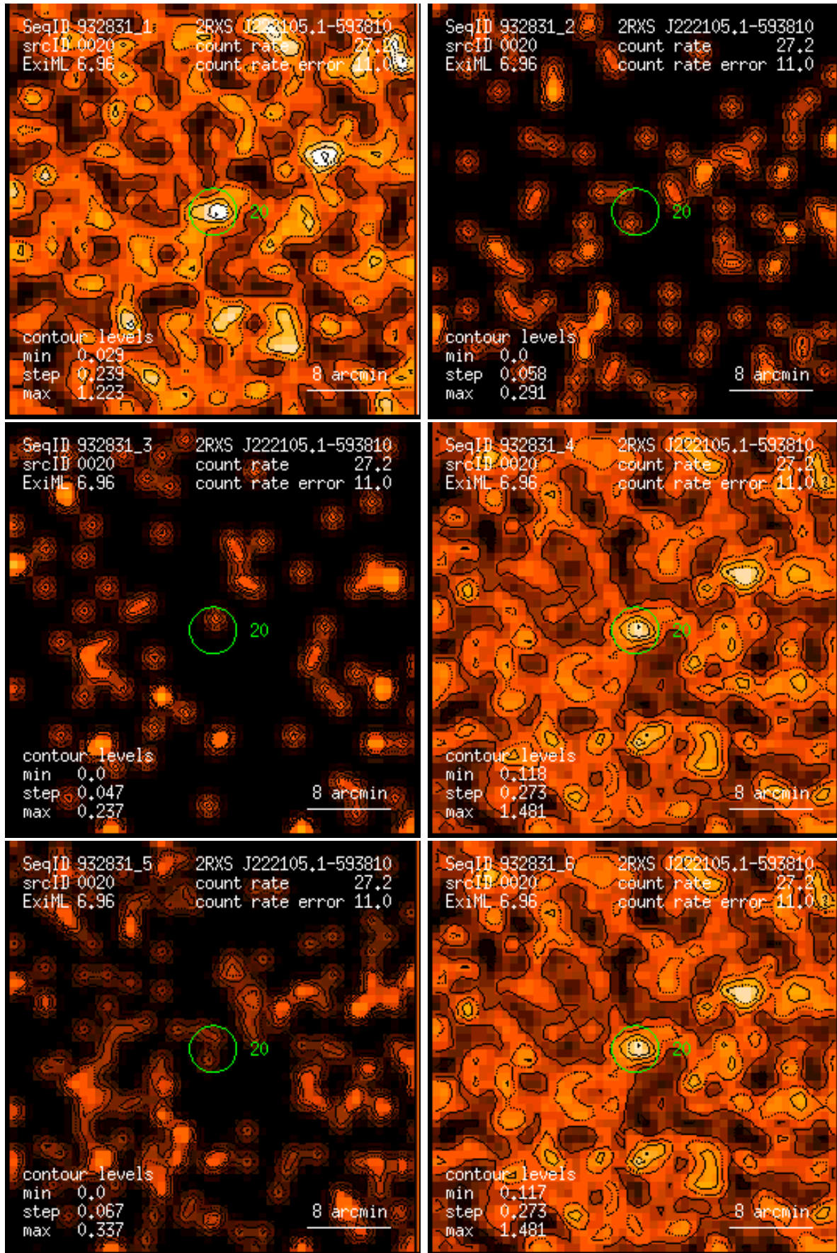
Figure 20: RASS 932831: detection 0020: band rate images, Gaussian filter: (1) PSPC channels 11 – 41, (2) 52 – 90, (3) 91 – 201, (4) 11 – 235, (5) 52 – 201, (6) 11 – 201. Broad band rates in counts/ks. Band rate contour levels in counts/ks/arcmin 2 .
