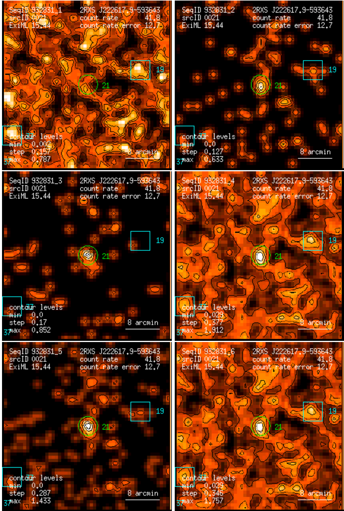
Figure 21: RASS 932831: detection 0021: band rate images, Gaussian filter: (1) PSPC channels 11 – 41, (2) 52 – 90, (3) 91 – 201, (4) 11 – 235, (5) 52 – 201, (6) 11 – 201. Broad band rates in counts/ks. Band rate contour levels in counts/ks/arcmin 2 .
