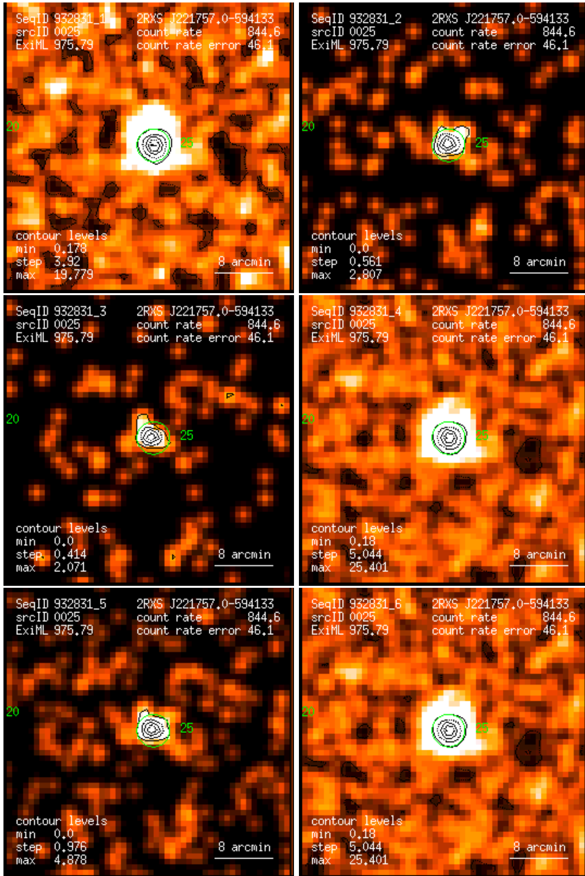
Figure 25: RASS 932831: detection 0025: band rate images, Gaussian filter: (1) PSPC channels 11 – 41, (2) 52 – 90, (3) 91 – 201, (4) 11 – 235, (5) 52 – 201, (6) 11 – 201. Broad band rates in counts/ks. Band rate contour levels in counts/ks/arcmin 2 .
