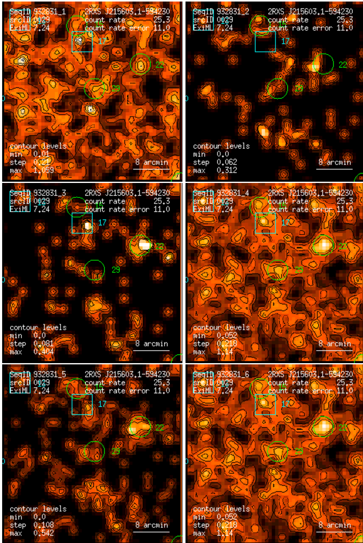
Figure 29: RASS 932831: detection 0029: band rate images, Gaussian filter: (1) PSPC channels 11 – 41, (2) 52 – 90, (3) 91 – 201, (4) 11 – 235, (5) 52 – 201, (6) 11 – 201. Broad band rates in counts/ks. Band rate contour levels in counts/ks/arcmin 2 .
