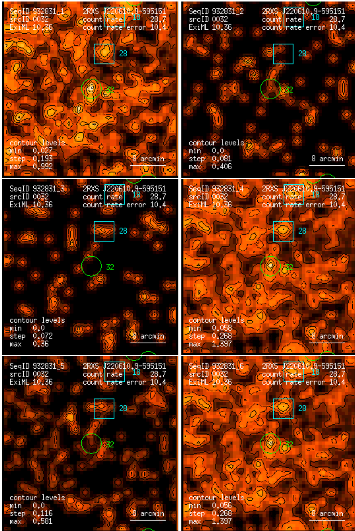
Figure 32: RASS 932831: detection 0032: band rate images, Gaussian filter: (1) PSPC channels 11 – 41, (2) 52 – 90, (3) 91 – 201, (4) 11 – 235, (5) 52 – 201, (6) 11 – 201. Broad band rates in counts/ks. Band rate contour levels in counts/ks/arcmin 2 .
