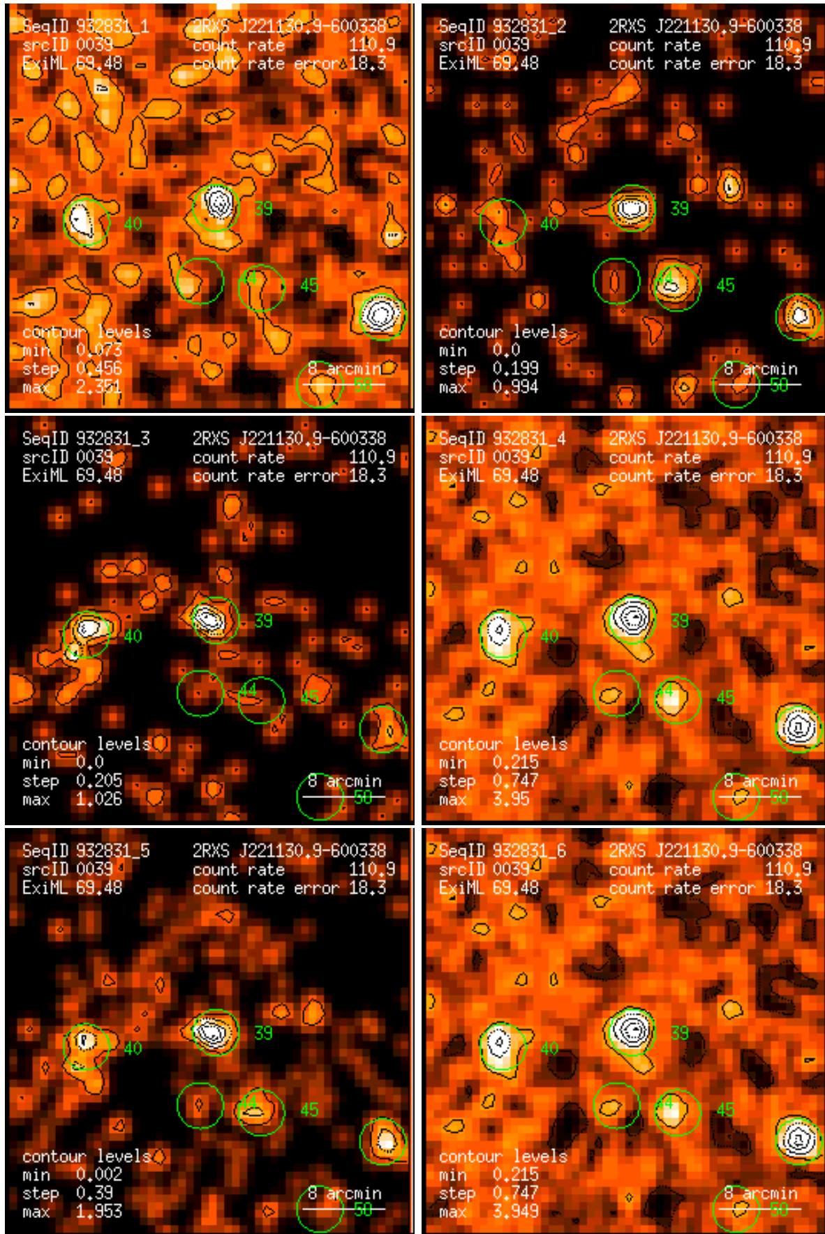
Figure 39: RASS 932831: detection 0039: band rate images, Gaussian filter: (1) PSPC channels 11 – 41, (2) 52 – 90, (3) 91 – 201, (4) 11 – 235, (5) 52 – 201, (6) 11 – 201. Broad band rates in counts/ks. Band rate contour levels in counts/ks/arcmin 2 .
