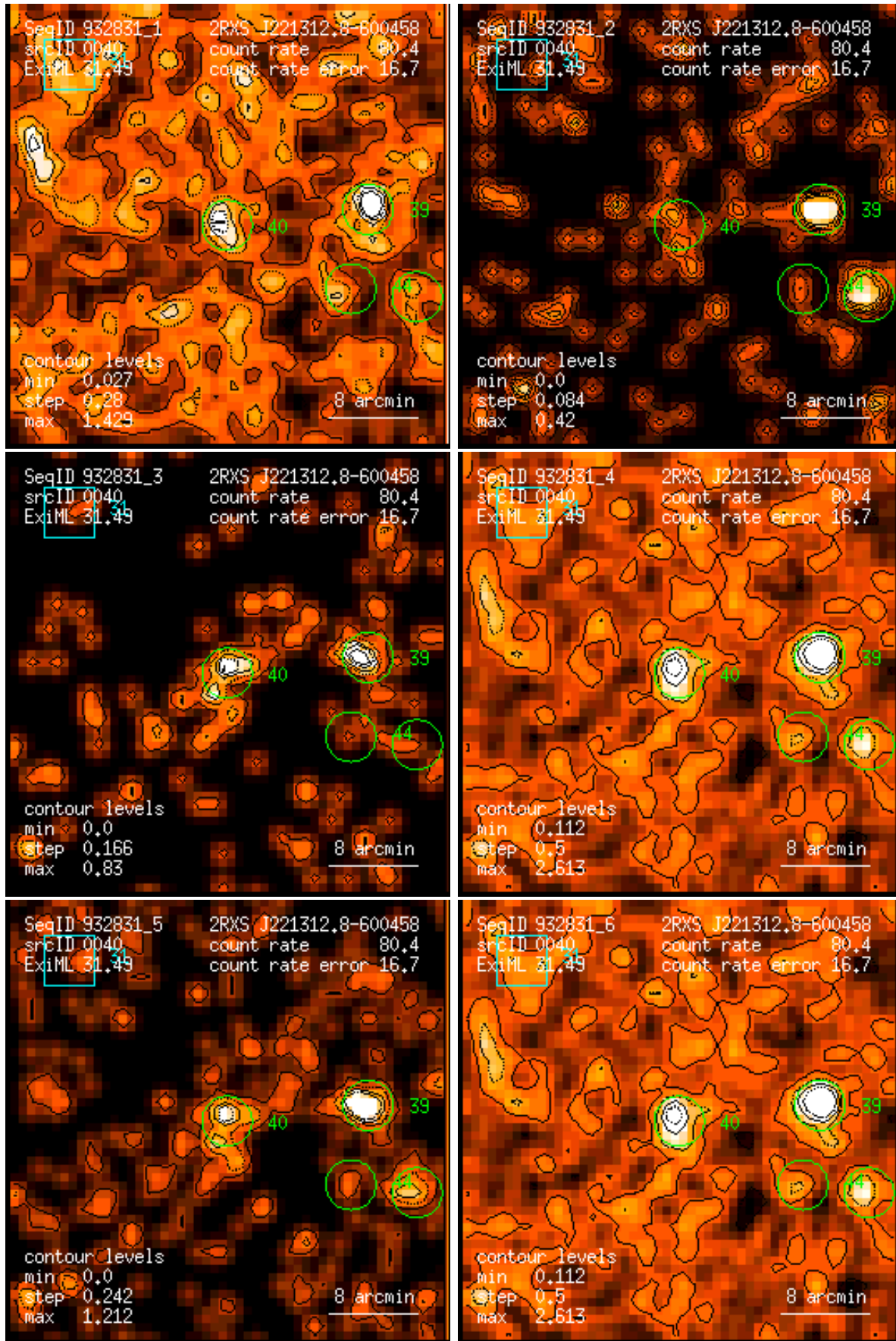
Figure 40: RASS 932831: detection 0040: band rate images, Gaussian filter: (1) PSPC channels 11 – 41, (2) 52 – 90, (3) 91 – 201, (4) 11 – 235, (5) 52 – 201, (6) 11 – 201. Broad band rates in counts/ks. Band rate contour levels in counts/ks/arcmin 2 .
