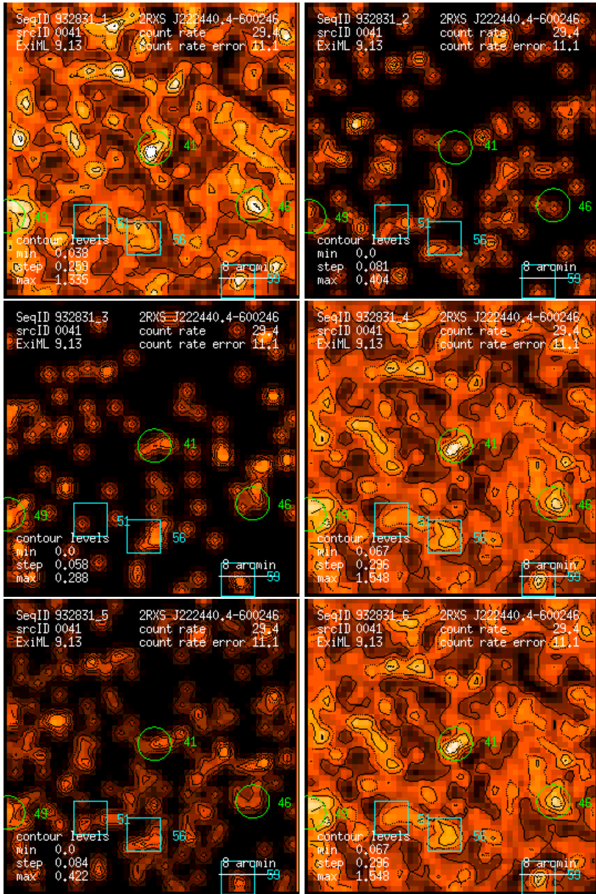
Figure 41: RASS 932831: detection 0041: band rate images, Gaussian filter: (1) PSPC channels 11 – 41, (2) 52 – 90, (3) 91 – 201, (4) 11 – 235, (5) 52 – 201, (6) 11 – 201. Broad band rates in counts/ks. Band rate contour levels in counts/ks/arcmin 2 .
