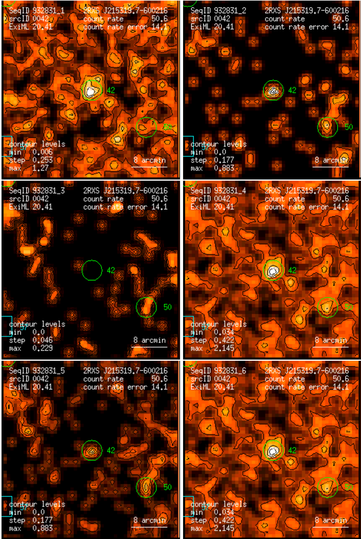
Figure 42: RASS 932831: detection 0042: band rate images, Gaussian filter: (1) PSPC channels 11 – 41, (2) 52 – 90, (3) 91 – 201, (4) 11 – 235, (5) 52 – 201, (6) 11 – 201. Broad band rates in counts/ks. Band rate contour levels in counts/ks/arcmin 2 .
