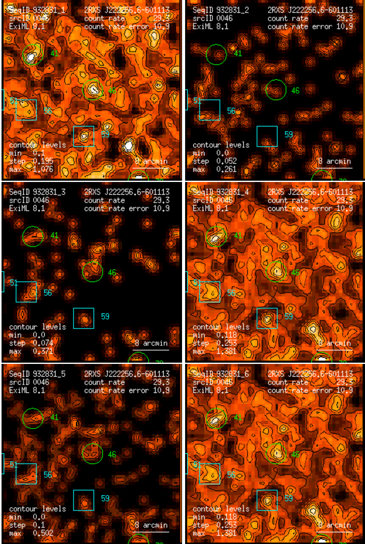
Figure 46: RASS 932831: detection 0046: band rate images, Gaussian filter: (1) PSPC channels 11 – 41, (2) 52 – 90, (3) 91 – 201, (4) 11 – 235, (5) 52 – 201, (6) 11 – 201. Broad band rates in counts/ks. Band rate contour levels in counts/ks/arcmin 2 .
