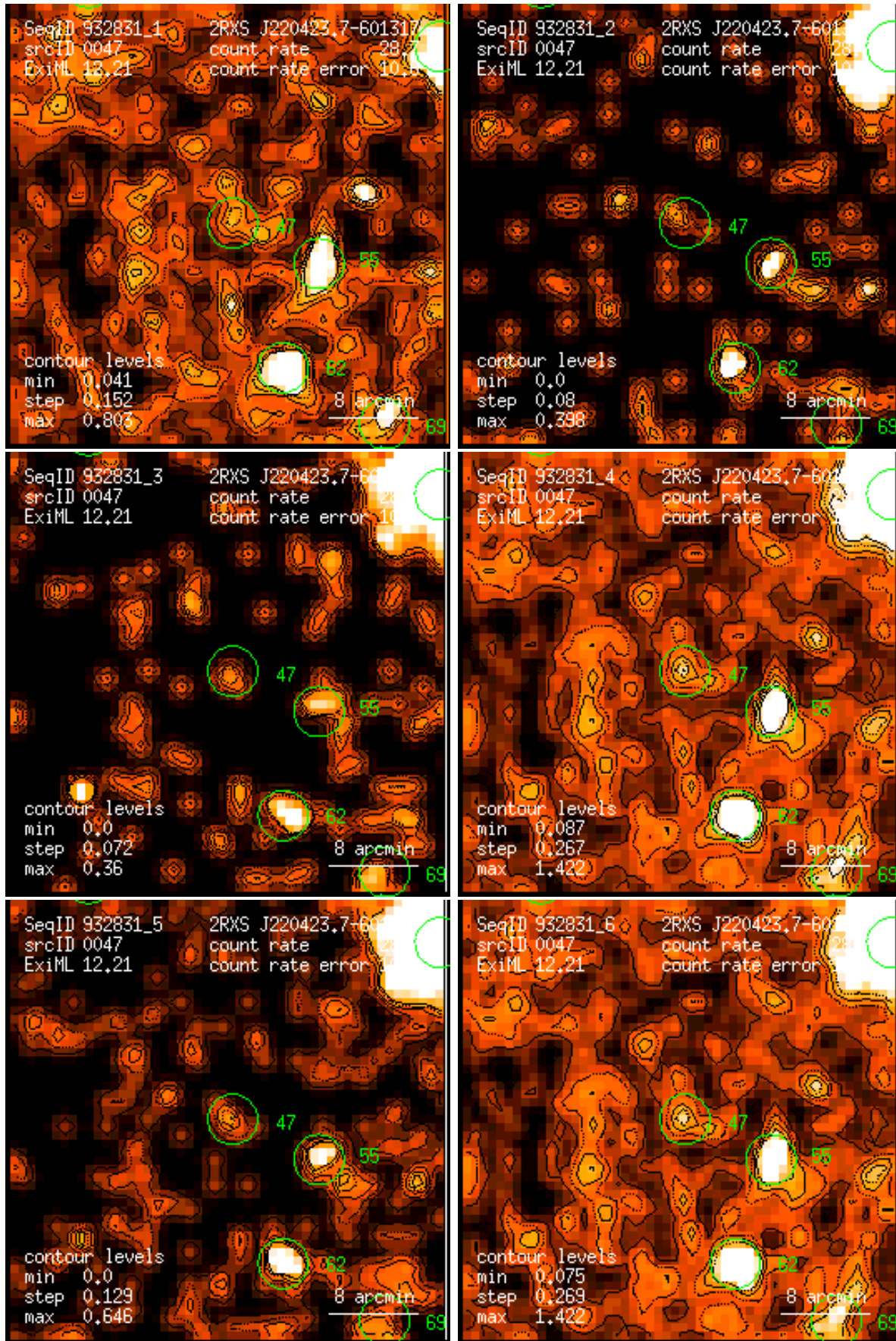
Figure 47: RASS 932831: detection 0047: band rate images, Gaussian filter: (1) PSPC channels 11 – 41, (2) 52 – 90, (3) 91 – 201, (4) 11 – 235, (5) 52 – 201, (6) 11 – 201. Broad band rates in counts/ks. Band rate contour levels in counts/ks/arcmin 2 .
