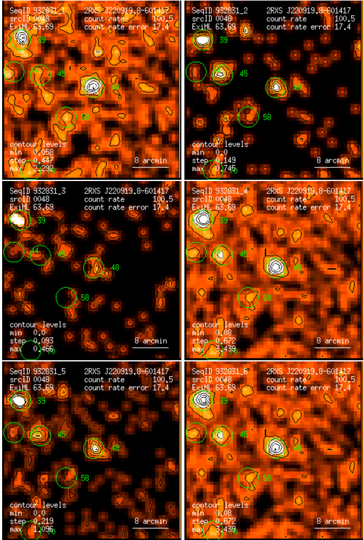
Figure 48: RASS 932831: detection 0048: band rate images, Gaussian filter: (1) PSPC channels 11 – 41, (2) 52 – 90, (3) 91 – 201, (4) 11 – 235, (5) 52 – 201, (6) 11 – 201. Broad band rates in counts/ks. Band rate contour levels in counts/ks/arcmin 2 .
