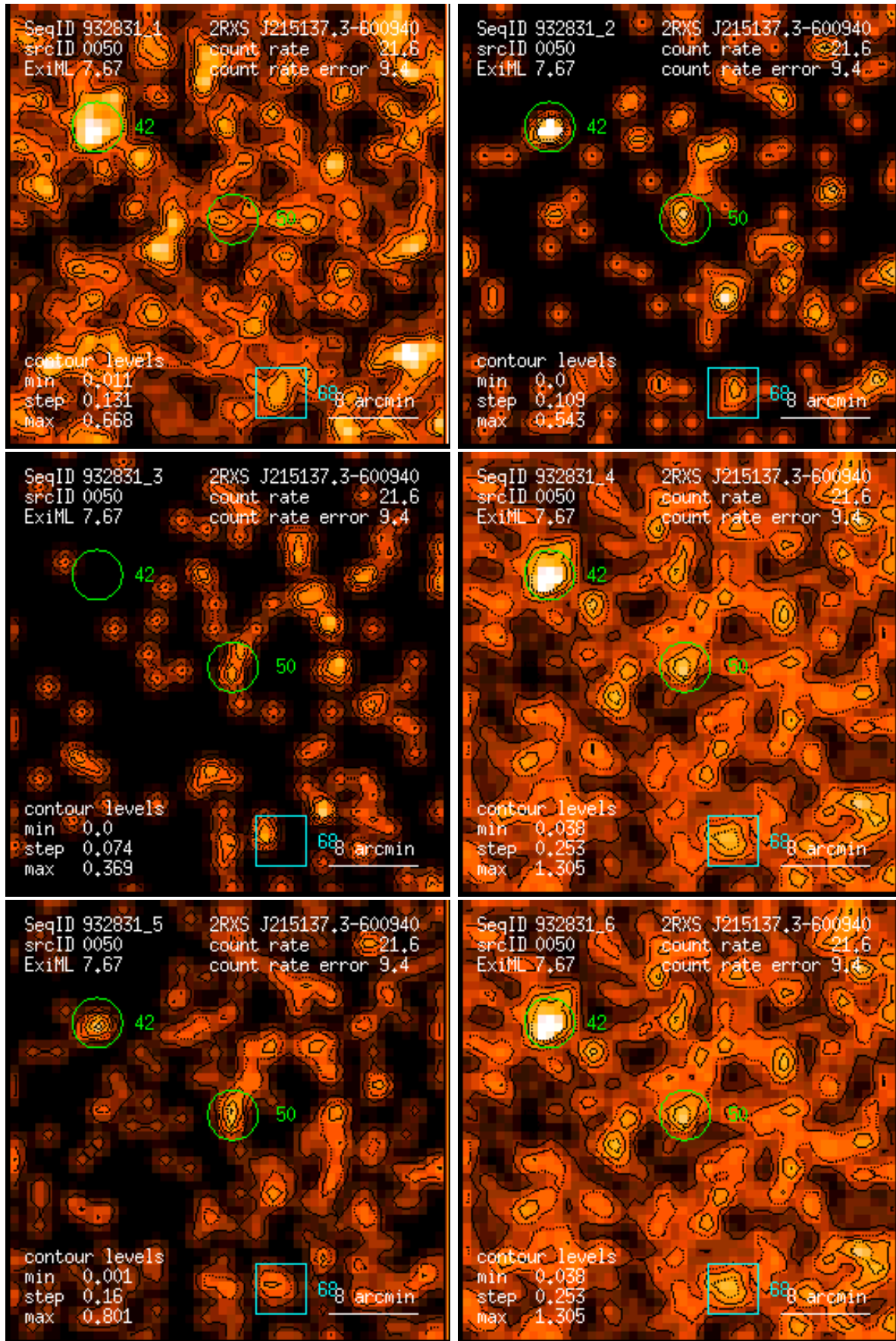
Figure 50: RASS 932831: detection 0050: band rate images, Gaussian filter: (1) PSPC channels 11 – 41, (2) 52 – 90, (3) 91 – 201, (4) 11 – 235, (5) 52 – 201, (6) 11 – 201. Broad band rates in counts/ks. Band rate contour levels in counts/ks/arcmin 2 .
