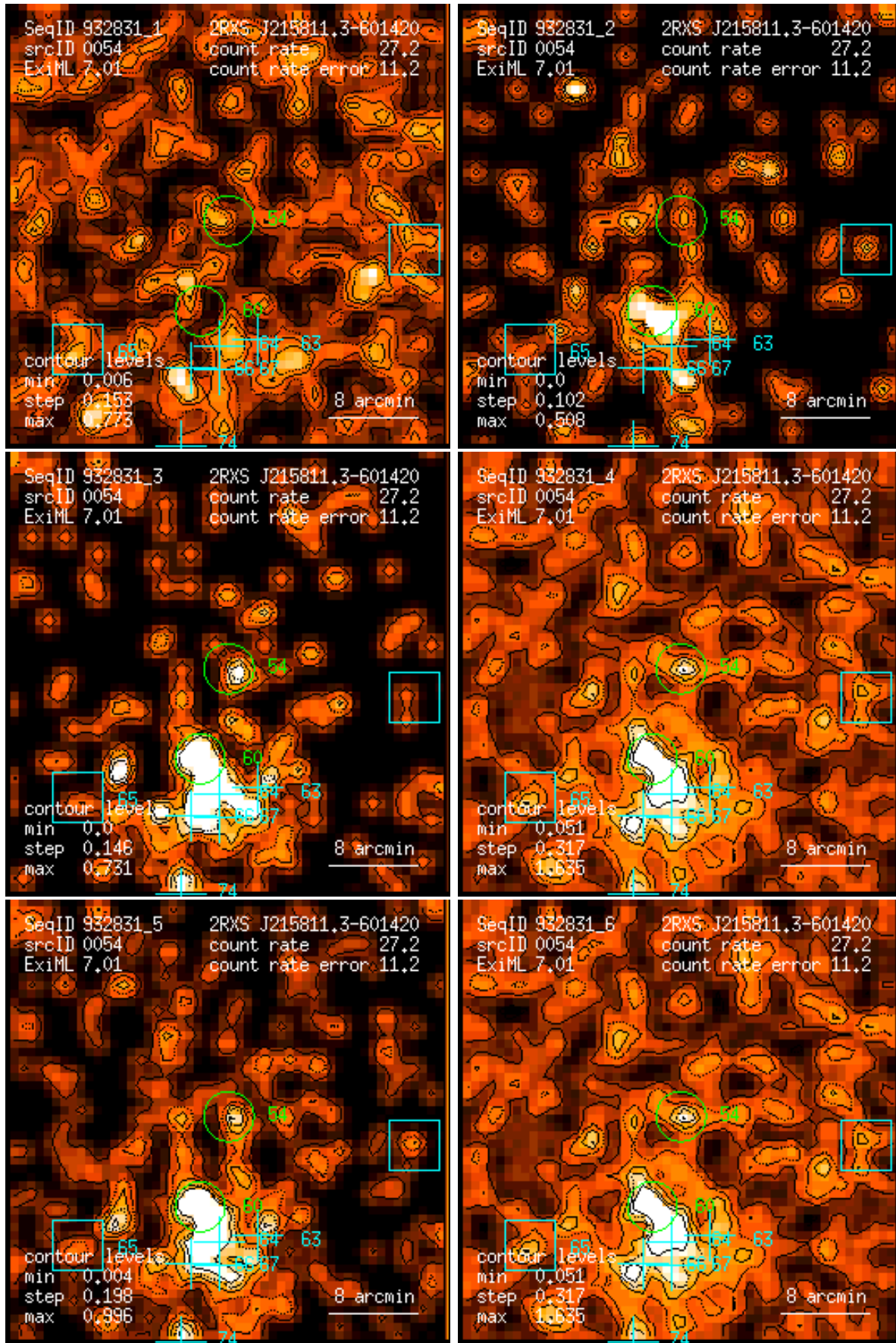
Figure 54: RASS 932831: detection 0054: band rate images, Gaussian filter: (1) PSPC channels 11 – 41, (2) 52 – 90, (3) 91 – 201, (4) 11 – 235, (5) 52 – 201, (6) 11 – 201. Broad band rates in counts/ks. Band rate contour levels in counts/ks/arcmin 2 .
