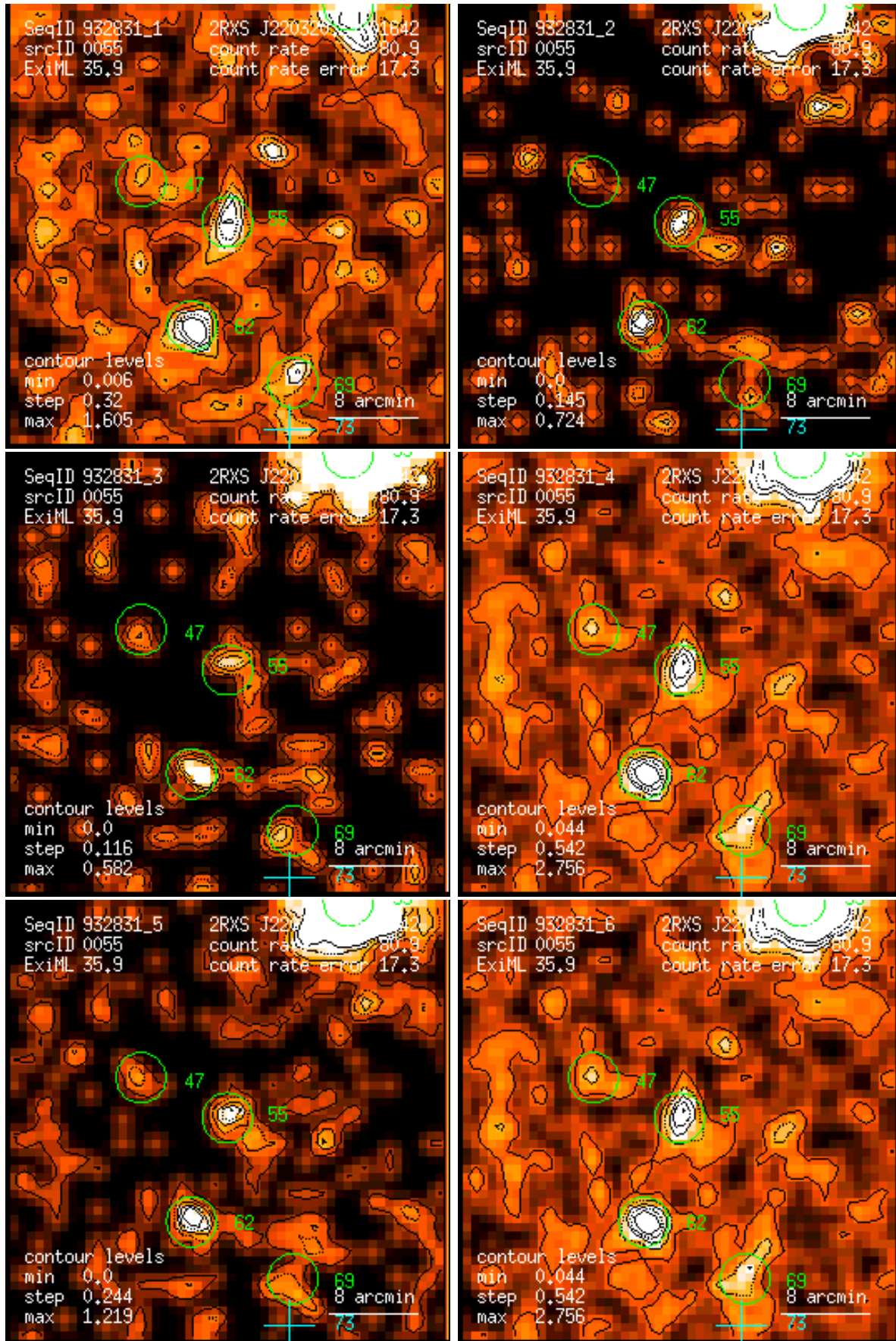
Figure 55: RASS 932831: detection 0055: band rate images, Gaussian filter: (1) PSPC channels 11 – 41, (2) 52 – 90, (3) 91 – 201, (4) 11 – 235, (5) 52 – 201, (6) 11 – 201. Broad band rates in counts/ks. Band rate contour levels in counts/ks/arcmin 2 .
