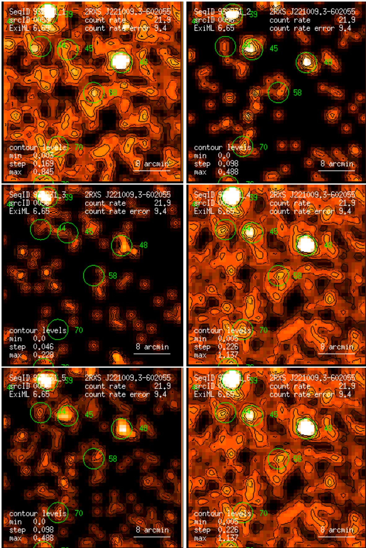
Figure 58: RASS 932831: detection 0058: band rate images, Gaussian filter: (1) PSPC channels 11 – 41, (2) 52 – 90, (3) 91 – 201, (4) 11 – 235, (5) 52 – 201, (6) 11 – 201. Broad band rates in counts/ks. Band rate contour levels in counts/ks/arcmin 2 .
