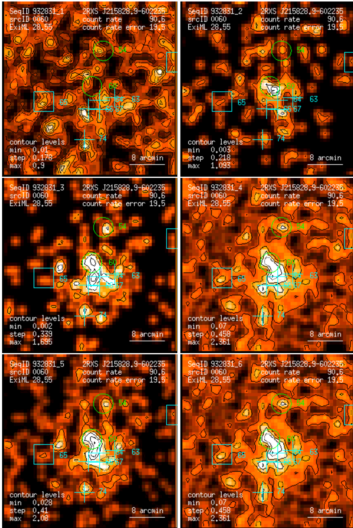
Figure 60: RASS 932831: detection 0060: band rate images, Gaussian filter: (1) PSPC channels 11 – 41, (2) 52 – 90, (3) 91 – 201, (4) 11 – 235, (5) 52 – 201, (6) 11 – 201. Broad band rates in counts/ks. Band rate contour levels in counts/ks/arcmin 2 .
