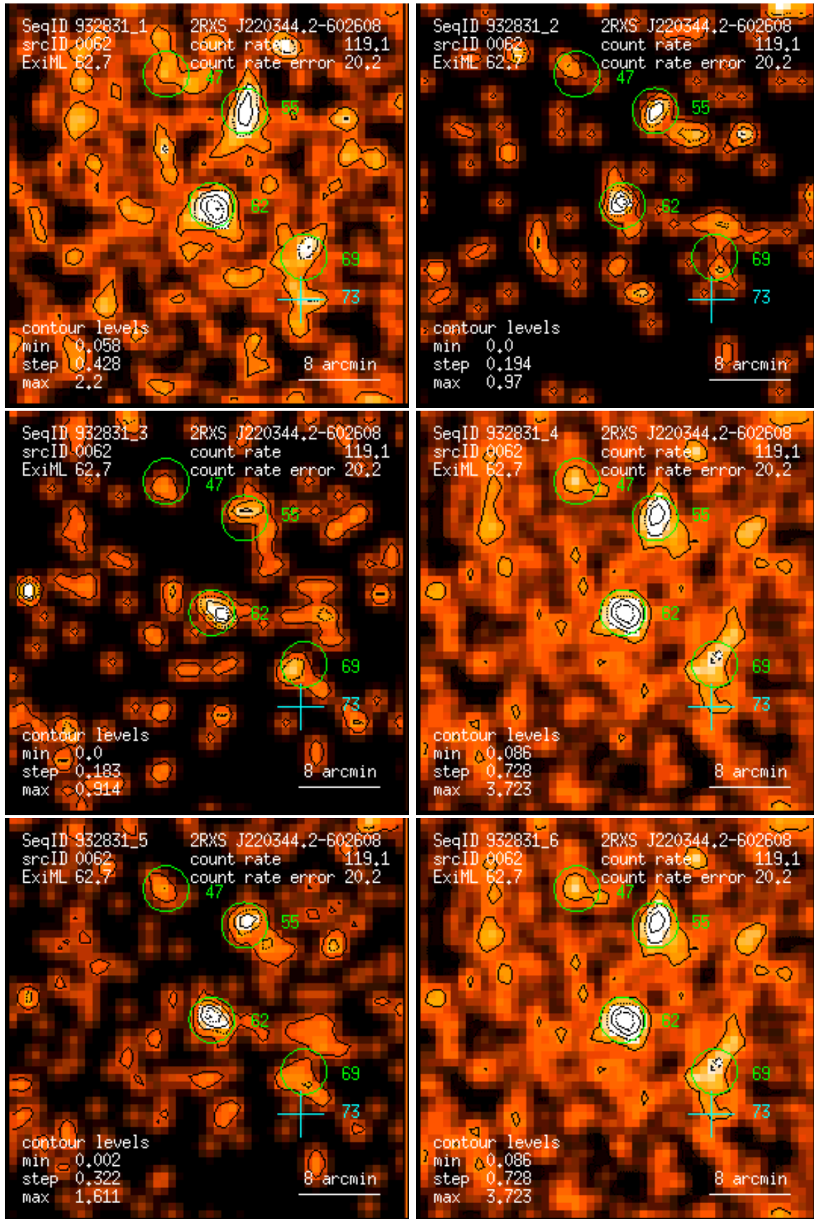
Figure 62: RASS 932831: detection 0062: band rate images, Gaussian filter: (1) PSPC channels 11 – 41, (2) 52 – 90, (3) 91 – 201, (4) 11 – 235, (5) 52 – 201, (6) 11 – 201. Broad band rates in counts/ks. Band rate contour levels in counts/ks/arcmin 2 .
