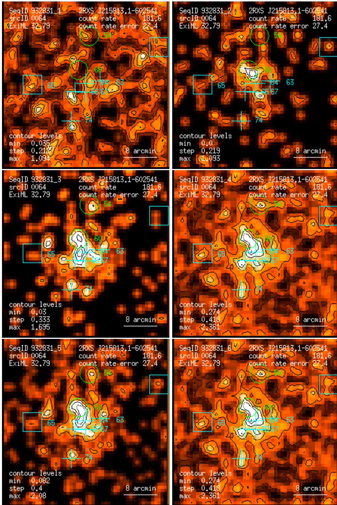
Figure 64: RASS 932831: detection 0064: band rate images, Gaussian filter: (1) PSPC channels 11 – 41, (2) 52 – 90, (3) 91 – 201, (4) 11 – 235, (5) 52 – 201, (6) 11 – 201. Broad band rates in counts/ks. Band rate contour levels in counts/ks/arcmin 2 .
