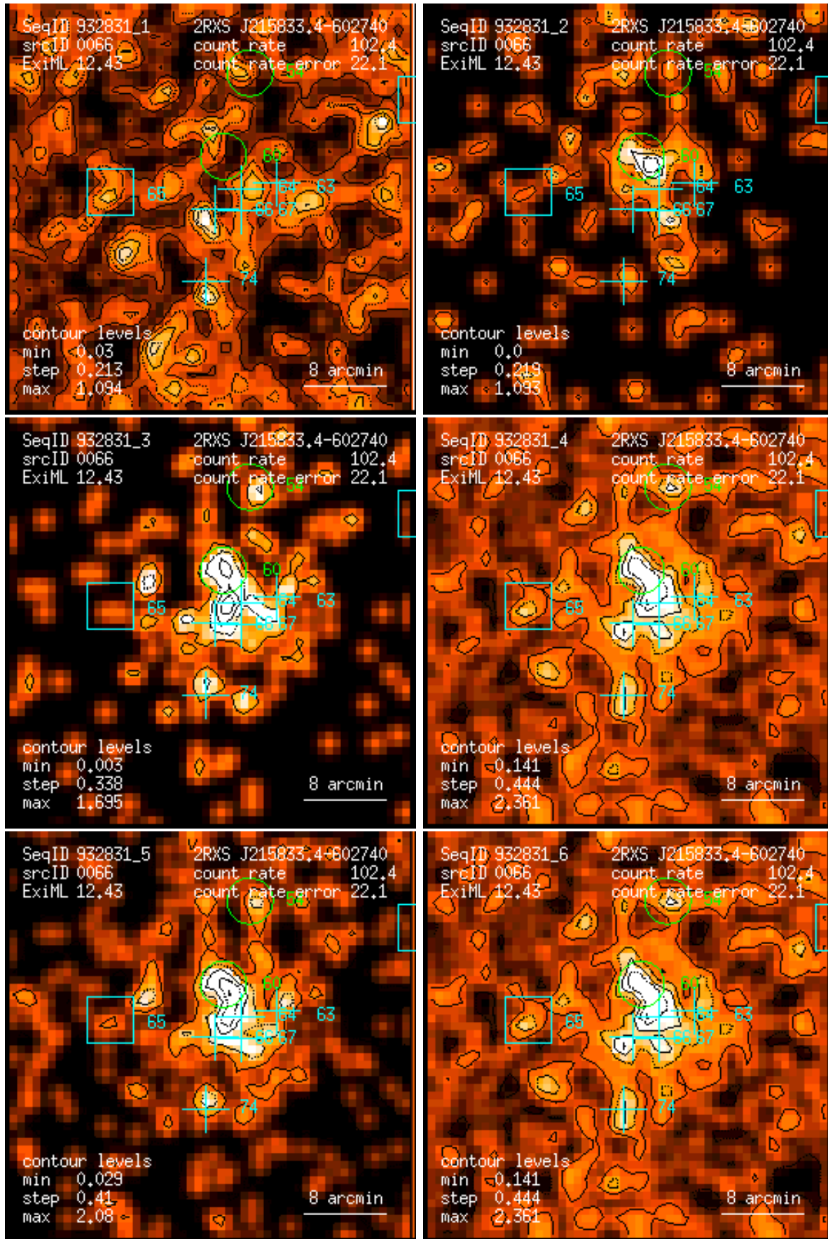
Figure 66: RASS 932831: detection 0066: band rate images, Gaussian filter: (1) PSPC channels 11 – 41, (2) 52 – 90, (3) 91 – 201, (4) 11 – 235, (5) 52 – 201, (6) 11 – 201. Broad band rates in counts/ks. Band rate contour levels in counts/ks/arcmin 2 .
