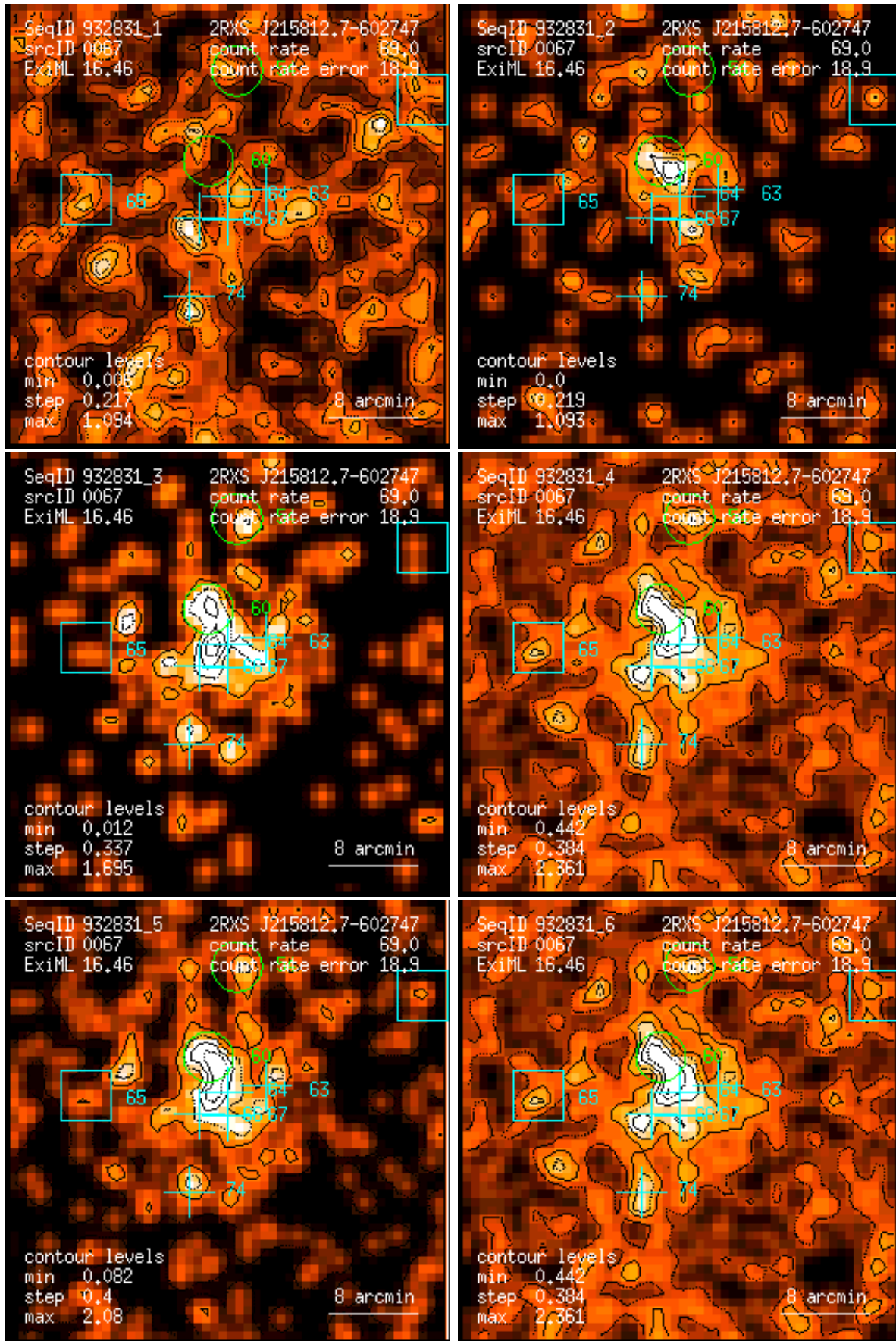
Figure 67: RASS 932831: detection 0067: band rate images, Gaussian filter: (1) PSPC channels 11 – 41, (2) 52 – 90, (3) 91 – 201, (4) 11 – 235, (5) 52 – 201, (6) 11 – 201. Broad band rates in counts/ks. Band rate contour levels in counts/ks/arcmin 2 .
