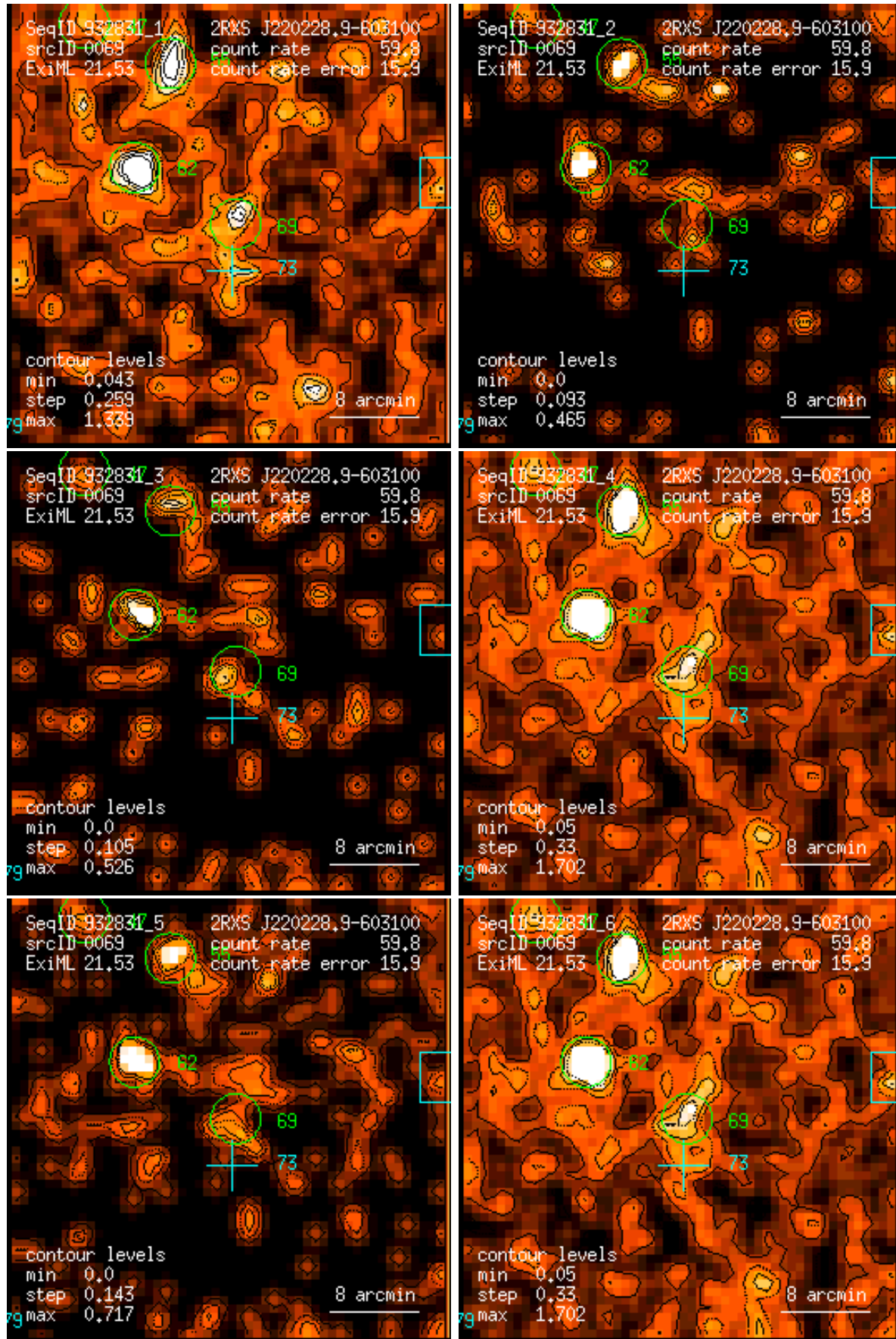
Figure 69: RASS 932831: detection 0069: band rate images, Gaussian filter: (1) PSPC channels 11 – 41, (2) 52 – 90, (3) 91 – 201, (4) 11 – 235, (5) 52 – 201, (6) 11 – 201. Broad band rates in counts/ks. Band rate contour levels in counts/ks/arcmin 2 .
