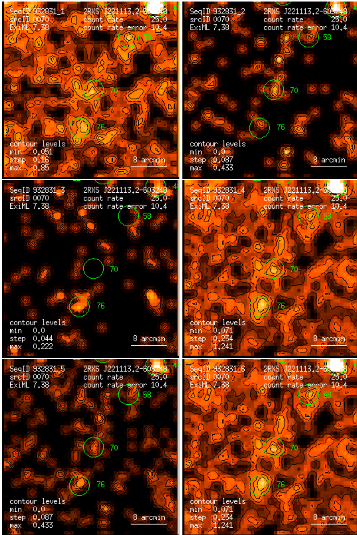
Figure 70: RASS 932831: detection 0070: band rate images, Gaussian filter: (1) PSPC channels 11 – 41, (2) 52 – 90, (3) 91 – 201, (4) 11 – 235, (5) 52 – 201, (6) 11 – 201. Broad band rates in counts/ks. Band rate contour levels in counts/ks/arcmin 2 .
